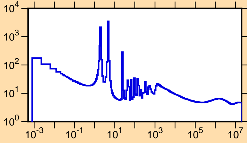
\sigma vs. E for ^{131}\text{Ba}(n,\text{tot.})
