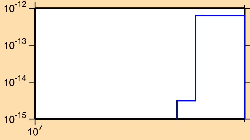
\sigma vs. E for ^{131}\text{Ba} (mt 45)
