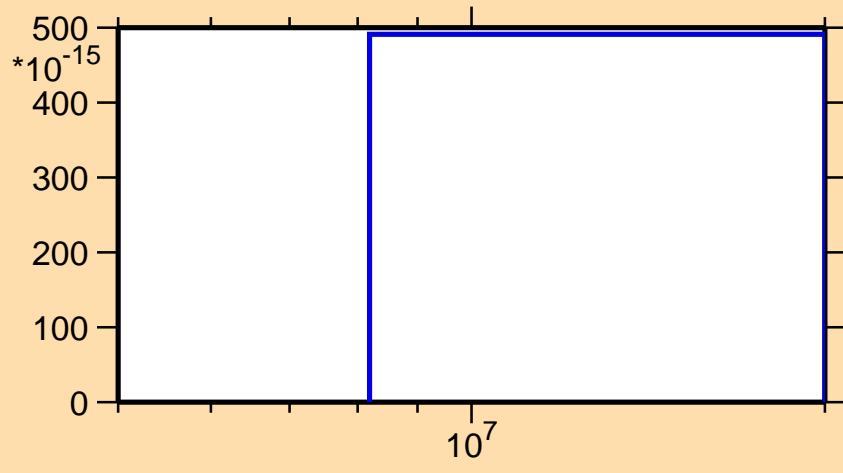
\sigma vs. E for ^{131}\text{Ba}(n,pd)
