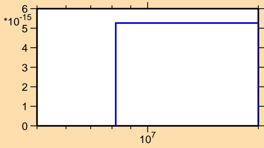
\sigma vs. E for ^{131}\text{Ba}(\text{mt117})
