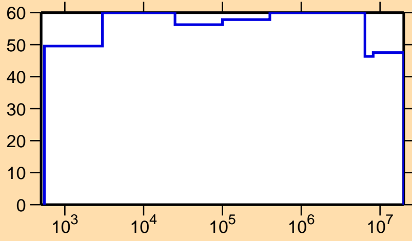
\Delta\sigma/\sigma vs. E for ^{131}\text{Ba}(n,p)
