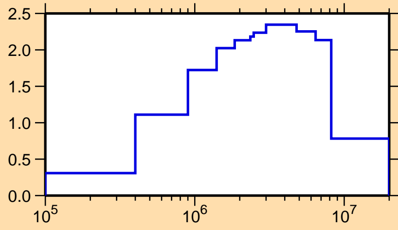
\sigma vs. E for ^{131}\text{Ba}(n,\text{inel.})
