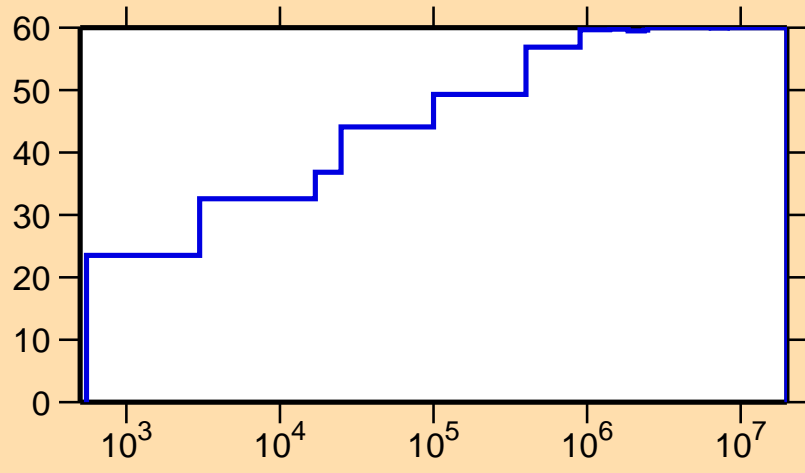
\Delta\sigma/\sigma vs. E for ^{131}\text{Ba}(n,\gamma)
