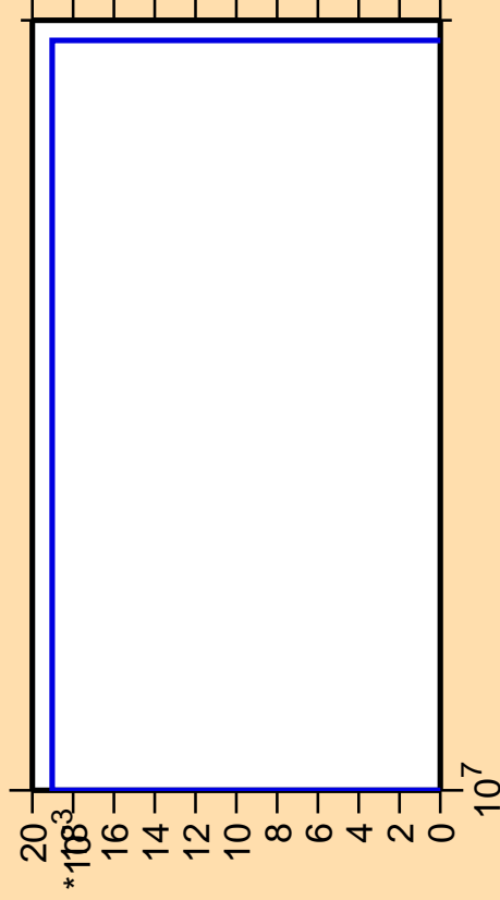
\Delta\sigma/\sigma vs. E for ^{131}\text{Ba} (mt 45)
