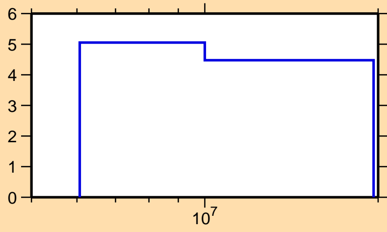
\Delta\sigma/\sigma vs. E for ^{131}\text{Ba}(n,\text{nonel.})
