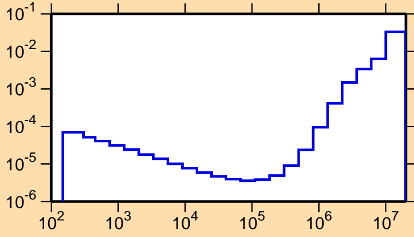
\sigma vs. E for ^{131}\text{Ba}(n,p)
