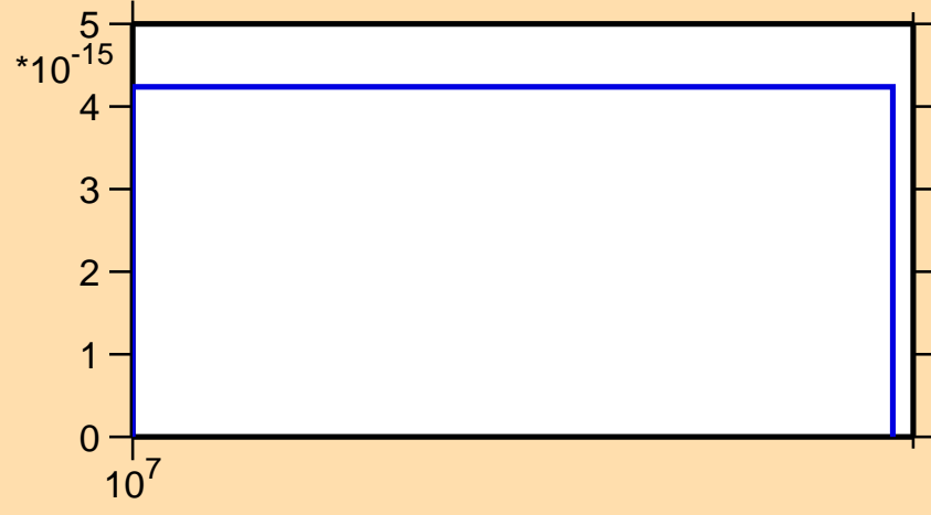
\sigma vs. E for ^{131}\text{Ba}(\text{mt117})
