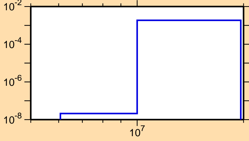
\sigma vs. E for ^{131}\text{Ba}(n,d)
