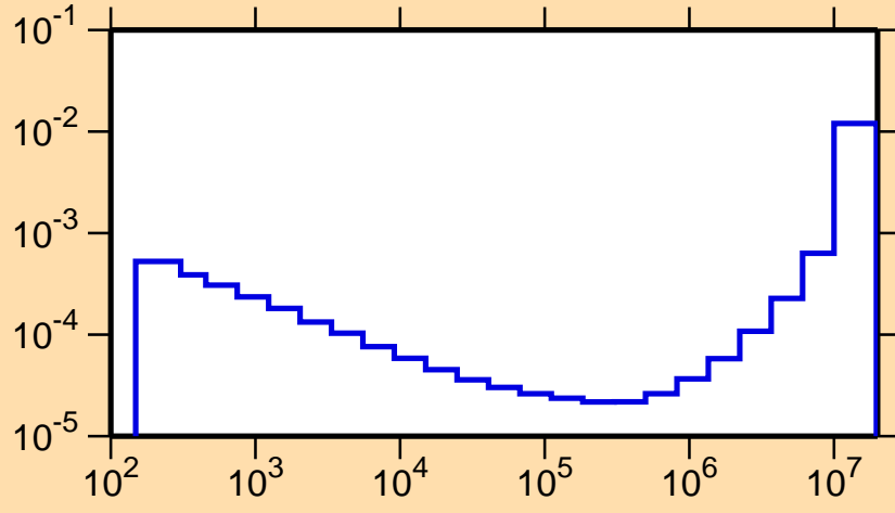
\sigma vs. E for ^{131}\text{Ba}(n,\alpha)
