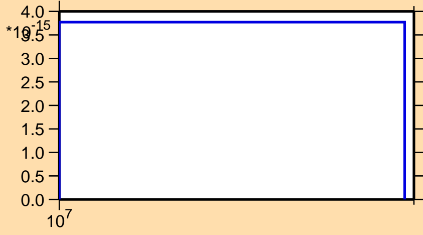
\sigma vs. E for ^{131}\text{Ba} (mt 45)
