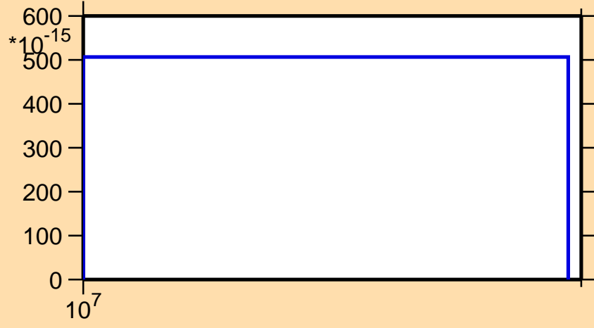
\sigma vs. E for ^{131}\text{Ba}(n,pd)
