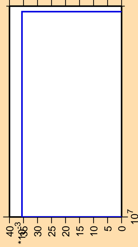
\Delta\sigma/\sigma vs. E for ^{131}\text{Ba}(\text{mt117})
