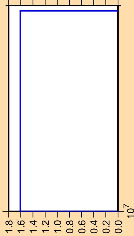
\Delta\sigma/\sigma vs. E for ^{131}\text{Ba}(n,pd)
