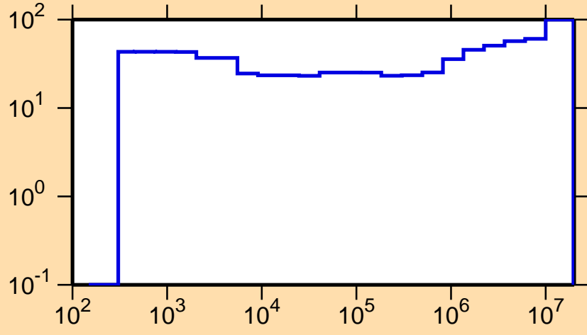
\Delta\sigma/\sigma vs. E for ^{131}\text{Ba}(n,\gamma)
