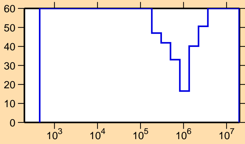
\Delta\sigma/\sigma vs. E for ^{131}\text{Ba}(n,n_1)
