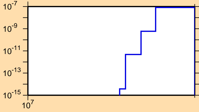
\sigma vs. E for ^{132}\text{Ba}(n,2n\alpha)
