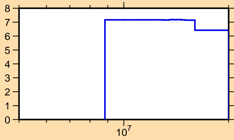
\Delta\sigma/\sigma vs. E for ^{132}\text{Ba}(n,\text{nonel.})
