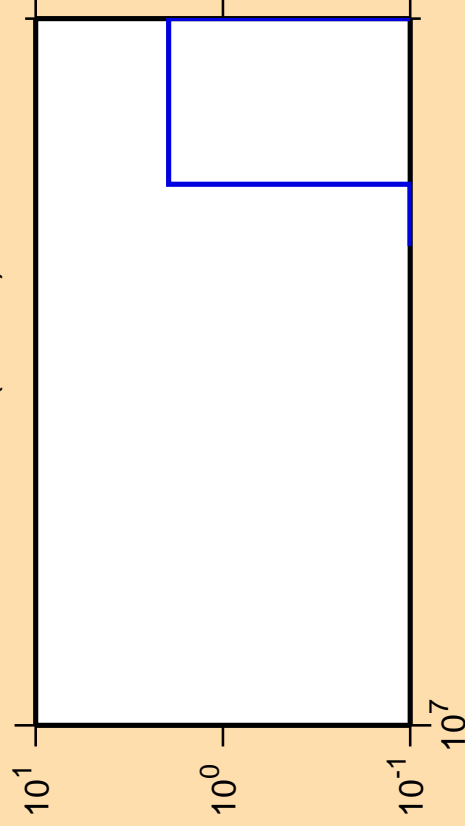
\Delta\sigma/\sigma vs. E for ^{132}\text{Ba} (mt 45)
