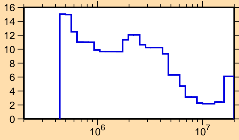
\Delta\sigma/\sigma vs. E for ^{132}\text{Ba}(n,\text{tot.})
