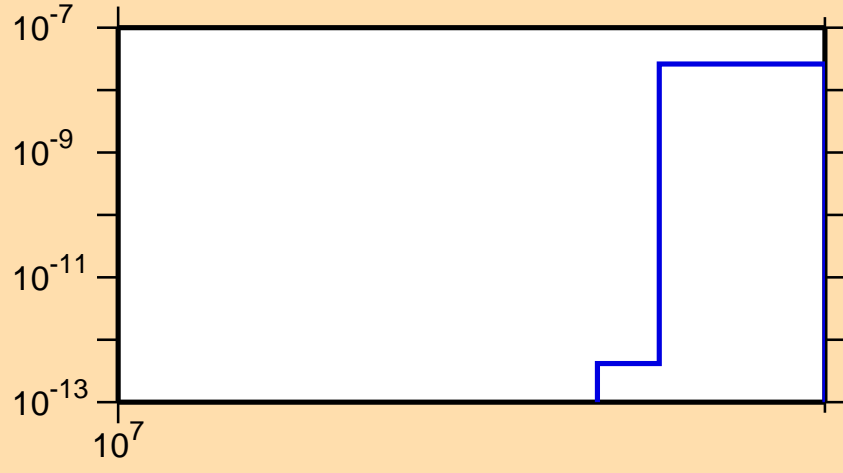
\sigma vs. E for ^{132}\text{Ba}(n,\text{nd})
