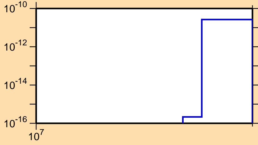
\sigma vs. E for ^{132}\text{Ba}(n,nt)
