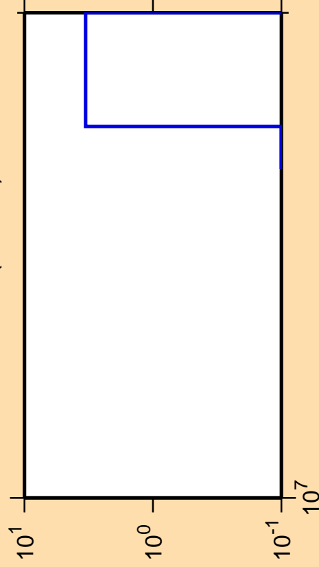
\Delta\sigma/\sigma vs. E for ^{132}\text{Ba}(\text{mt117})
