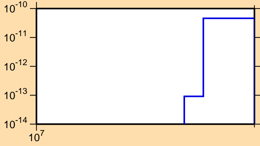
\sigma vs. E for ^{132}\text{Ba}(n,pd)
