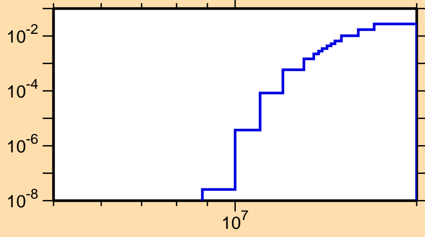
\sigma vs. E for ^{132}\text{Ba}(n,np)
