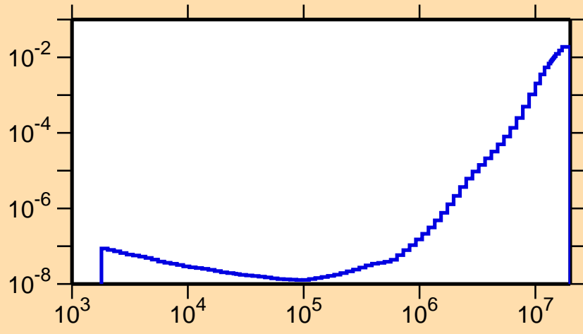
\sigma vs. E for ^{132}\text{Ba}(n,\alpha)
