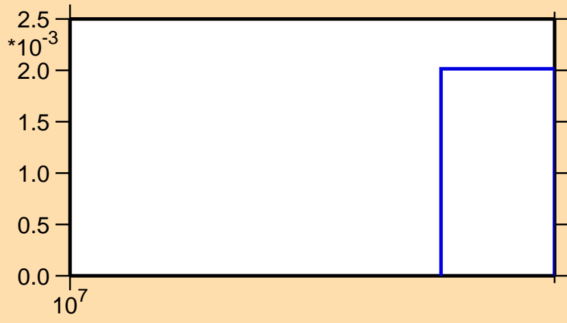
\sigma vs. E for ^{132}\text{Ba}(n,3n)
