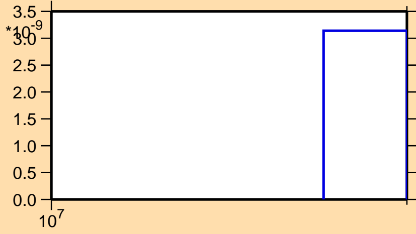
\sigma vs. E for ^{132}\text{Ba}(n,2np)
