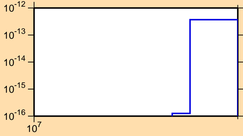
\sigma vs. E for ^{132}\text{Ba} (mt 45)
