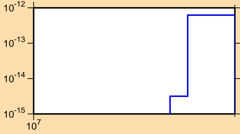
\sigma vs. E for ^{132}\text{Ba}(\text{mt117})
