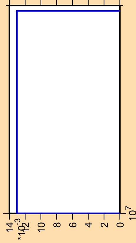
\Delta\sigma/\sigma vs. E for ^{132}\text{Ba} (mt 45)
