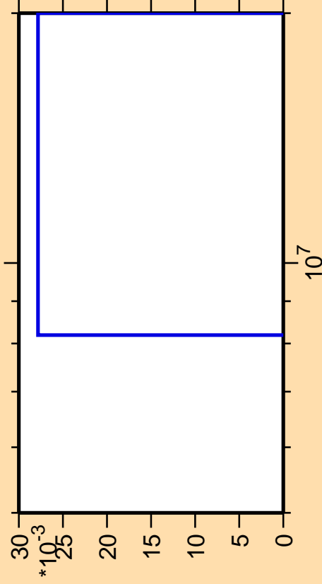
\Delta\sigma/\sigma vs. E for ^{132}\text{Ba}(\text{mt117})
