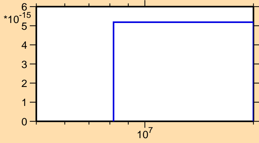
\sigma vs. E for ^{132}\text{Ba}(\text{mt117})
