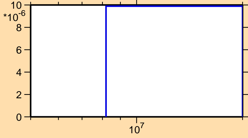
\sigma vs. E for ^{132}\text{Ba}(n,t)
