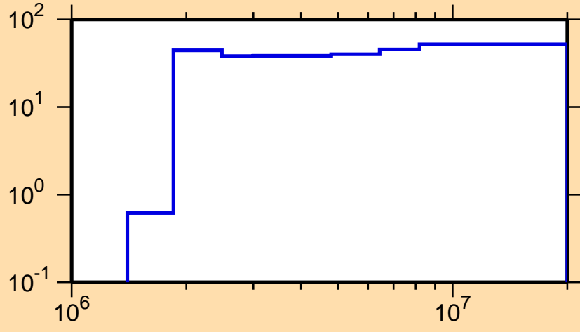
\Delta\sigma/\sigma vs. E for ^{132}\text{Ba}(n,p)
