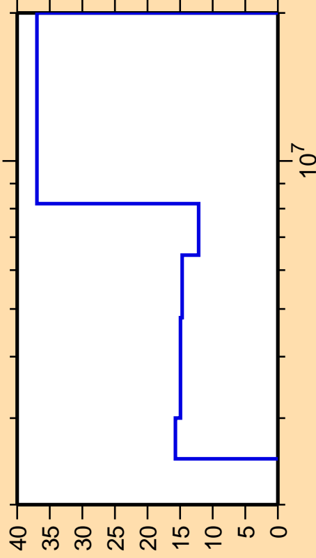
\Delta\sigma/\sigma vs. E for ^{132}\text{Ba}(n,n_{\text{cont}})
