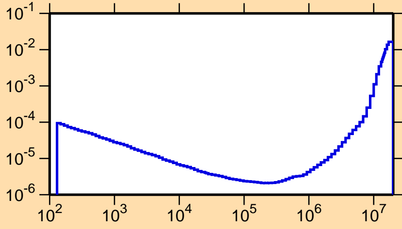
\sigma vs. E for ^{133}\text{Ba}(n,\alpha)
