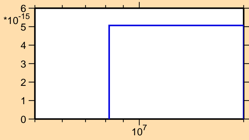
\sigma vs. E for ^{133}\text{Ba}(n,\text{pt})
