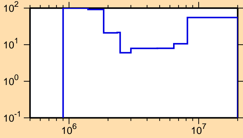
\Delta\sigma/\sigma vs. E for ^{133}\text{Ba}(n,n\text{cont.})
