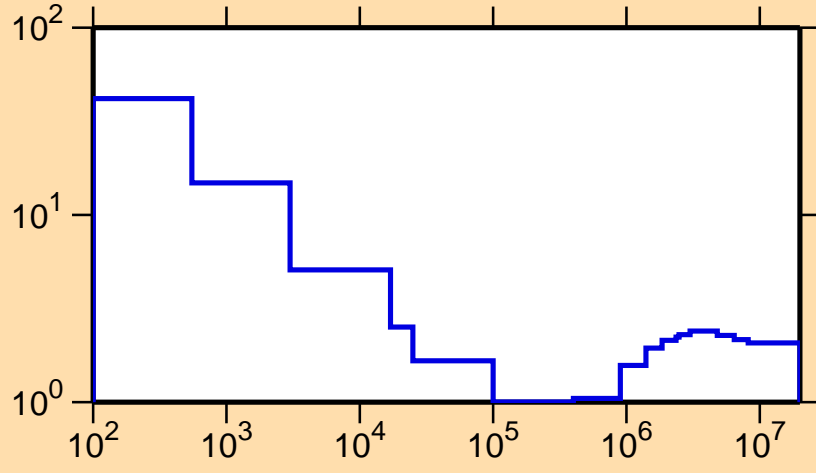
\sigma vs. E for ^{133}\text{Ba}(n,\text{nonel.})
