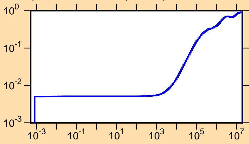
\mu vs. E for ^{134}\text{Ba}(\text{mt251})
