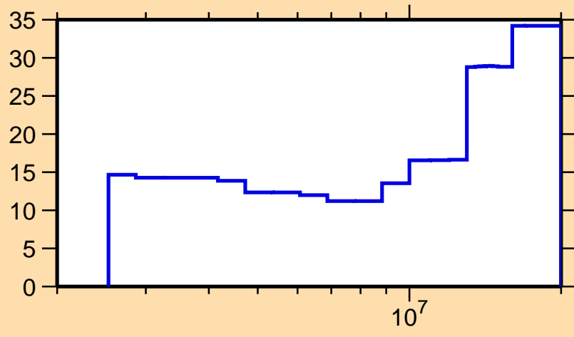
\Delta\sigma/\sigma vs. E for ^{134}\text{Ba}(n,n\text{cont.})
