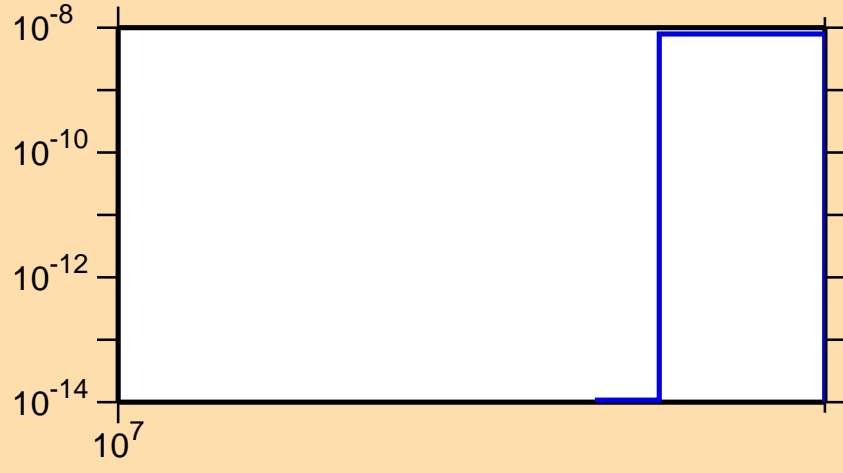
\sigma vs. E for ^{134}\text{Ba}(n,\text{nd})
