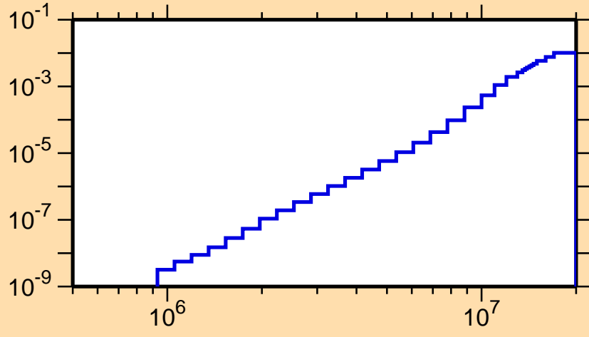
\sigma vs. E for ^{134}\text{Ba}(n,\alpha)
