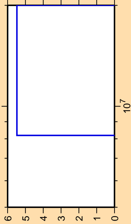
\Delta\sigma/\sigma vs. E for ^{134}\text{Ba}(n,p\alpha)
