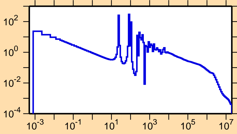
\sigma vs. E for ^{135}\text{Ba}(n,\gamma)
