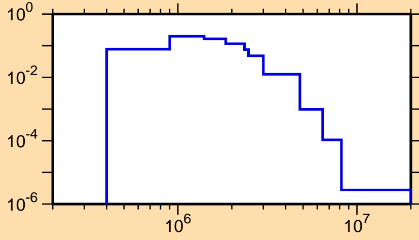
\sigma vs. E for ^{135}\text{Ba}(n,n_4)
