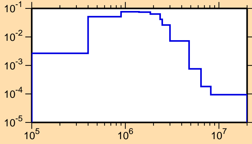
\sigma vs. E for ^{135}\text{Ba}(n,n_2)
