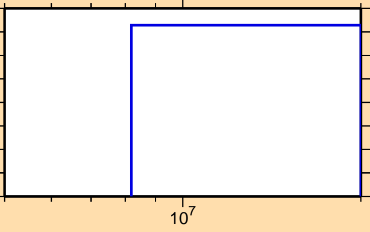
\sigma vs. E for ^{135}\text{Ba}(n,nt)
