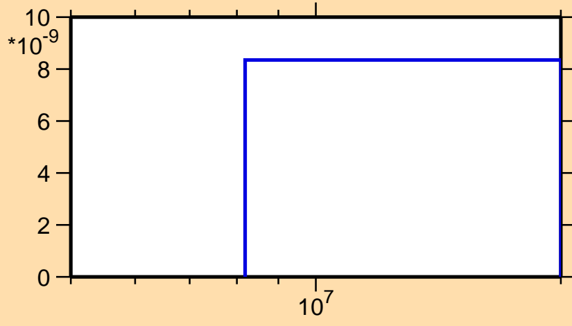
\sigma vs. E for ^{135}\text{Ba}(n,2n\alpha)
