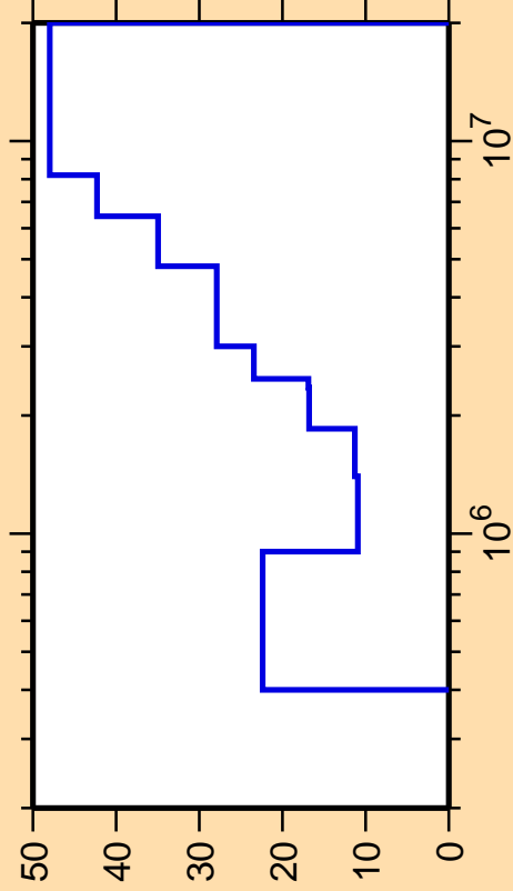
\Delta\sigma/\sigma vs. E for ^{135}\text{Ba}(n,n_4)
