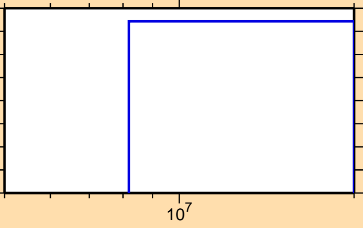
\sigma vs. E for ^{135}\text{Ba}(n,\text{nd})
