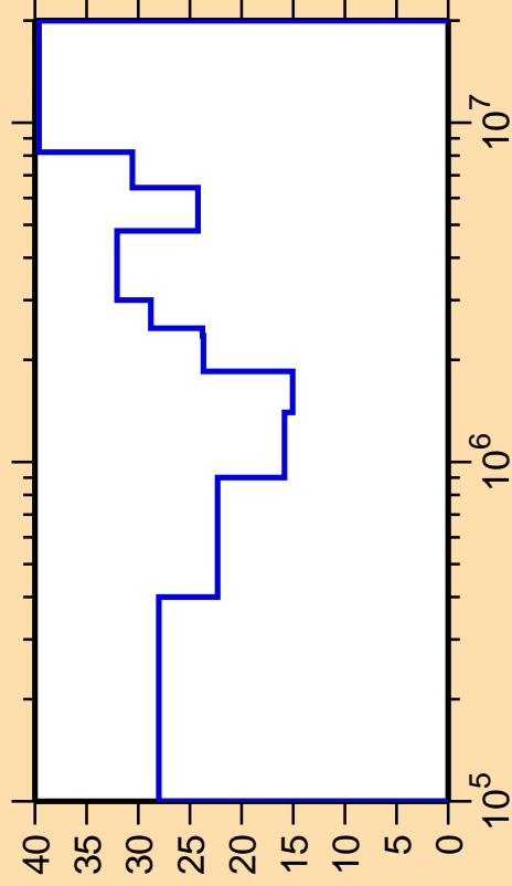
\Delta\sigma/\sigma vs. E for ^{135}\text{Ba}(n,n_2)
