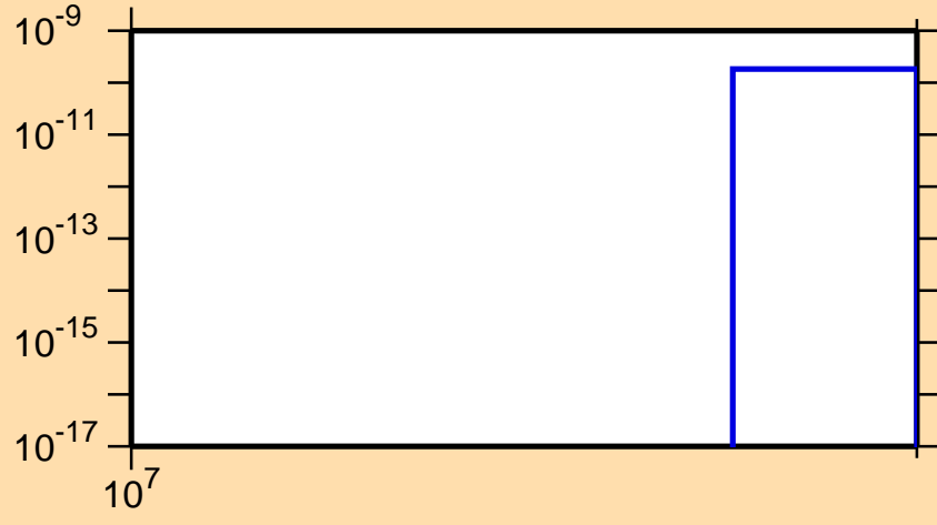
\sigma vs. E for ^{135}\text{Ba}(n,nt)
