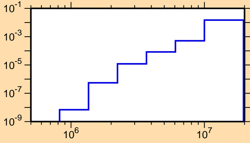
\sigma vs. E for ^{135}\text{Ba}(n,p)
