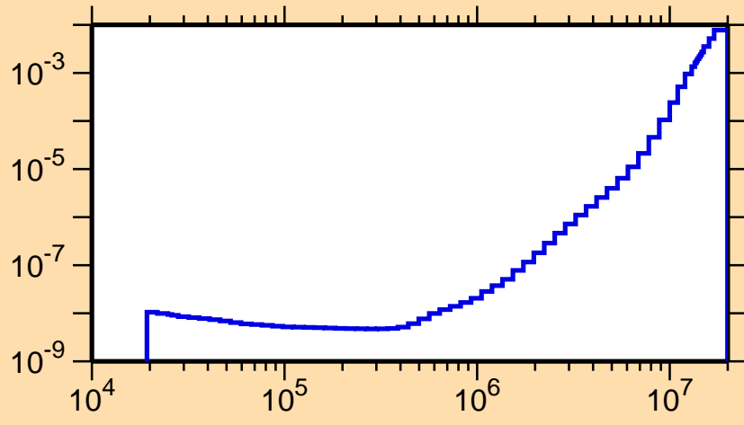
\sigma vs. E for ^{137}\text{Ba}(n,\alpha)
