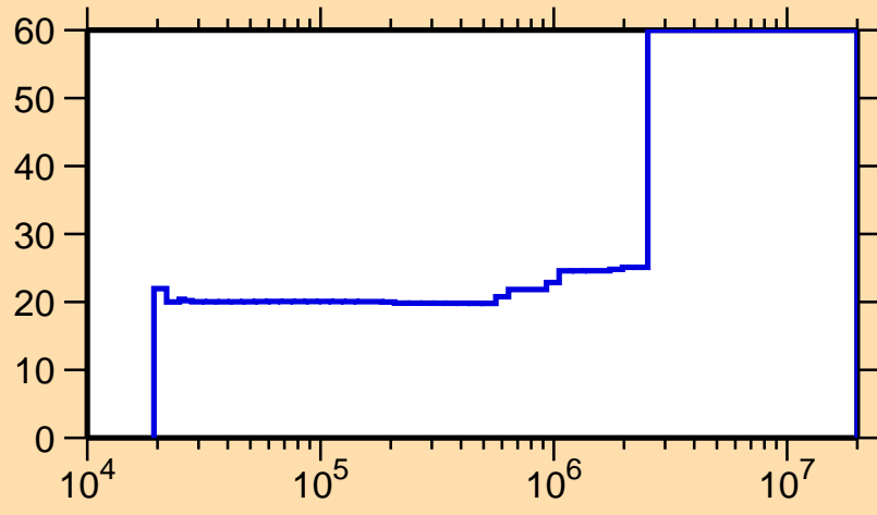
\Delta\sigma/\sigma vs. E for ^{137}\text{Ba}(n,\gamma)
