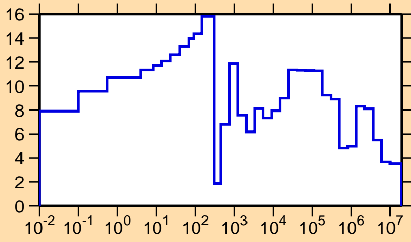
\Delta\sigma/\sigma vs. E for ^{137}\text{Ba}(n,\text{tot.})
