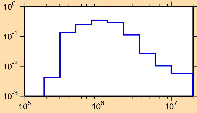
\sigma vs. E for ^{137}\text{Ba}(n,n_1)
