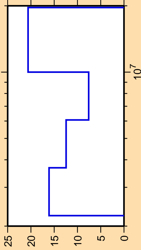
\Delta\sigma/\sigma vs. E for ^{137}\text{Ba}(n,n\text{cont.})
