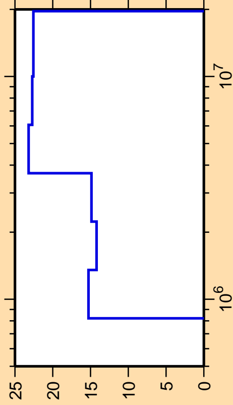
\Delta\sigma/\sigma vs. E for ^{137}\text{Ba}(n,n_3)
