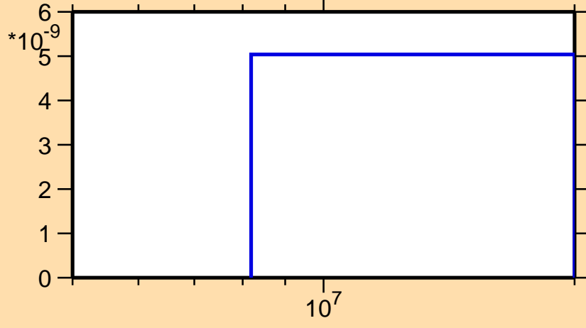
\sigma vs. E for ^{137}\text{Ba}(n,2n\alpha)
