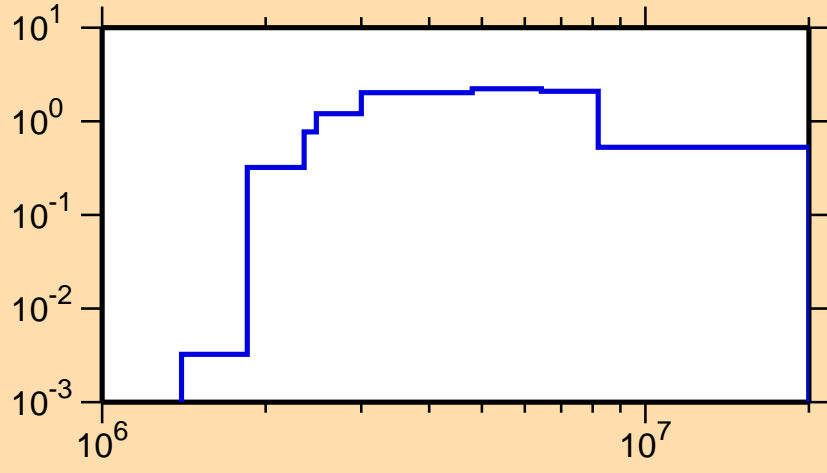
\sigma vs. E for ^{137}\text{Ba}(n,n\text{cont.})
