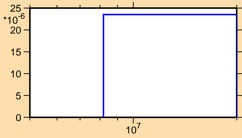
\sigma vs. E for ^{137}\text{Ba}(n,t)
