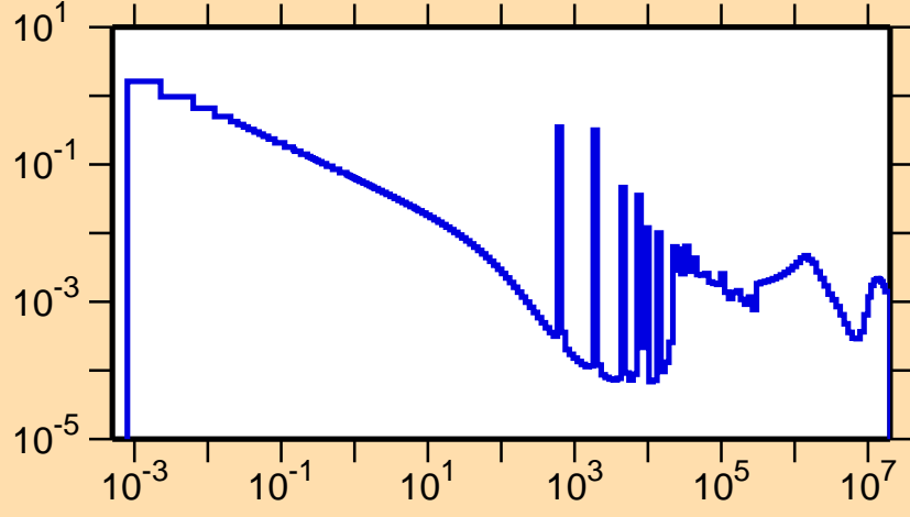
\sigma vs. E for ^{138}\text{Ba}(n,\gamma)
