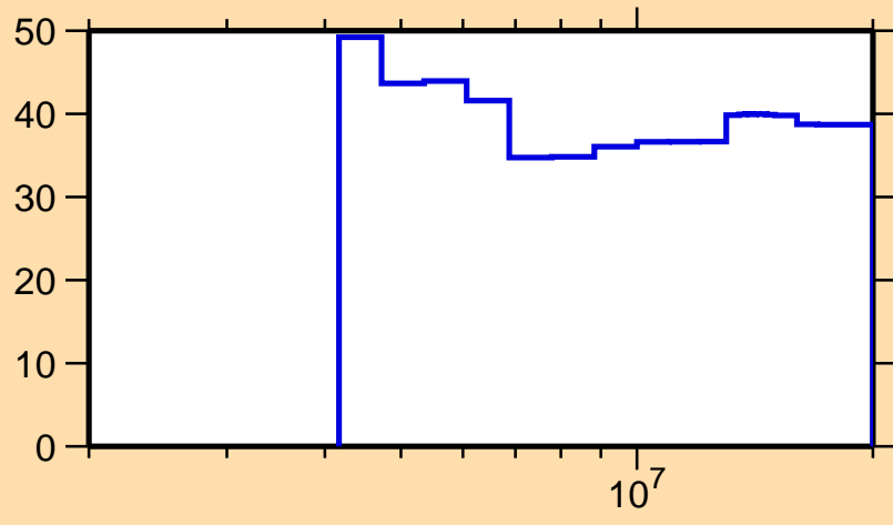
\Delta\sigma/\sigma vs. E for ^{139}\text{Ba}(n,n_1)
