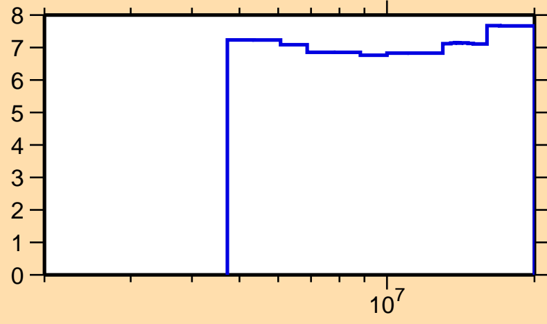
\Delta\sigma/\sigma vs. E for ^{139}\text{Ba}(n,\text{nonel.})
