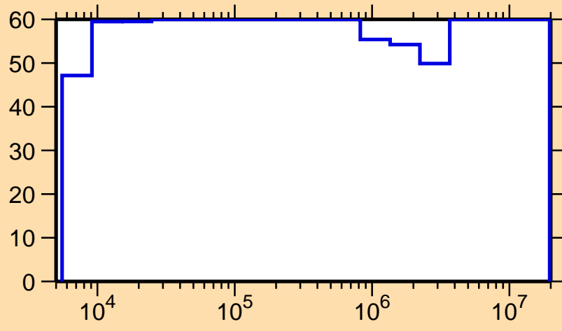
\Delta\sigma/\sigma vs. E for ^{139}\text{Ba}(n,\gamma)
