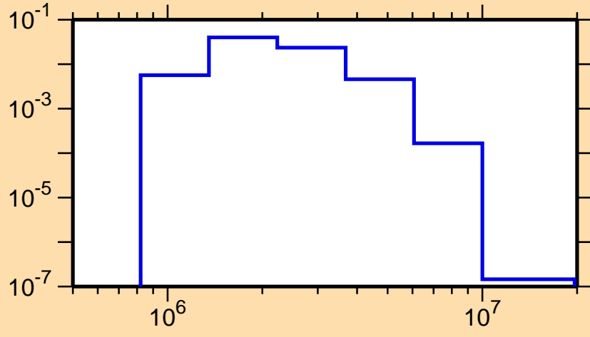
\sigma vs. E for ^{139}\text{Ba}(n,n_2)
