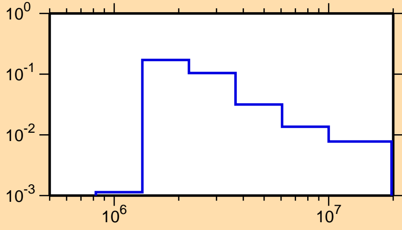
\sigma vs. E for ^{139}\text{Ba}(n,n_4)
