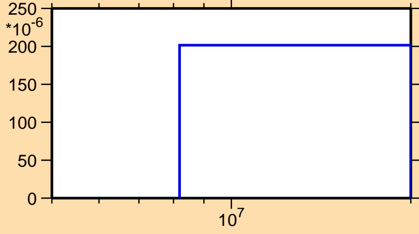
\sigma vs. E for ^{139}\text{Ba}(n,d)
