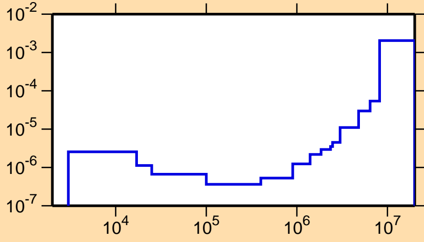
\sigma vs. E for ^{139}\text{Ba}(n,\alpha)
