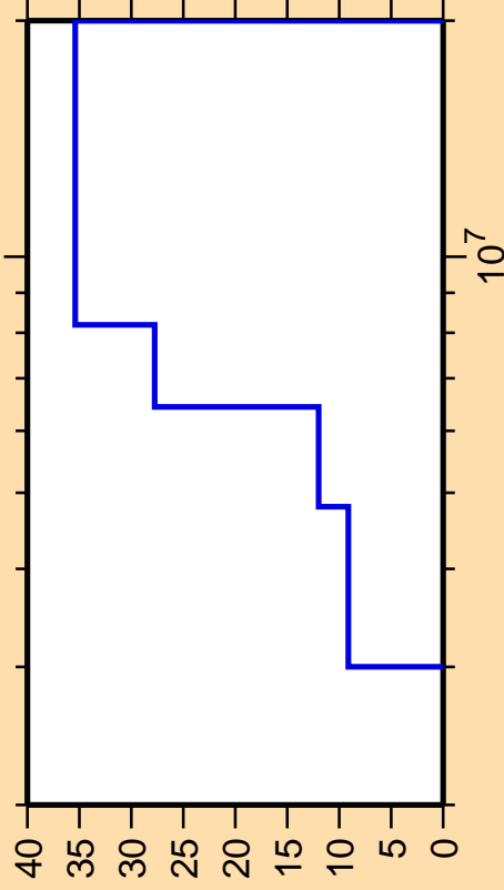
\Delta\sigma/\sigma vs. E for ^{139}\text{Ba}(n,n\text{cont.})
