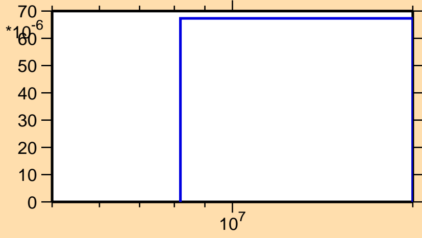
\sigma vs. E for ^{139}\text{Ba}(n,np)
