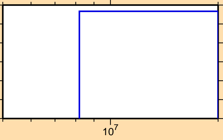
\sigma vs. E for ^{139}\text{Ba}(n,2np)
