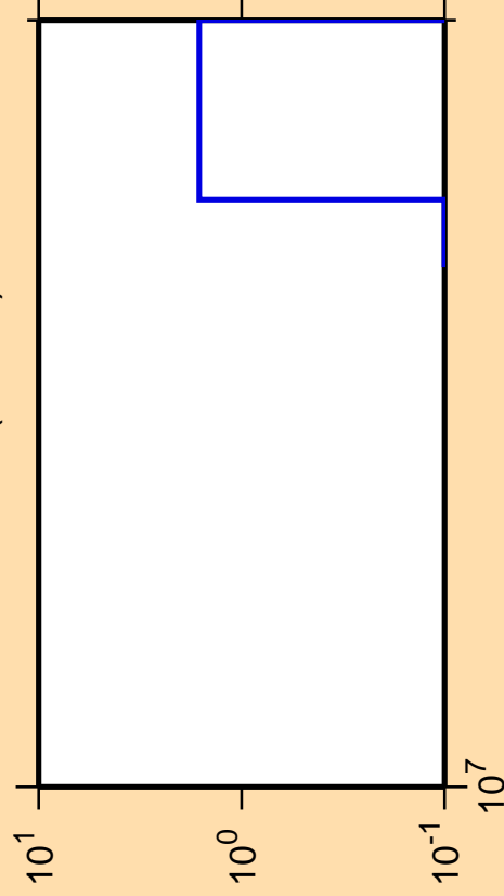
\Delta\sigma/\sigma vs. E for ^{140}\text{Ba}(n,3n\alpha)
