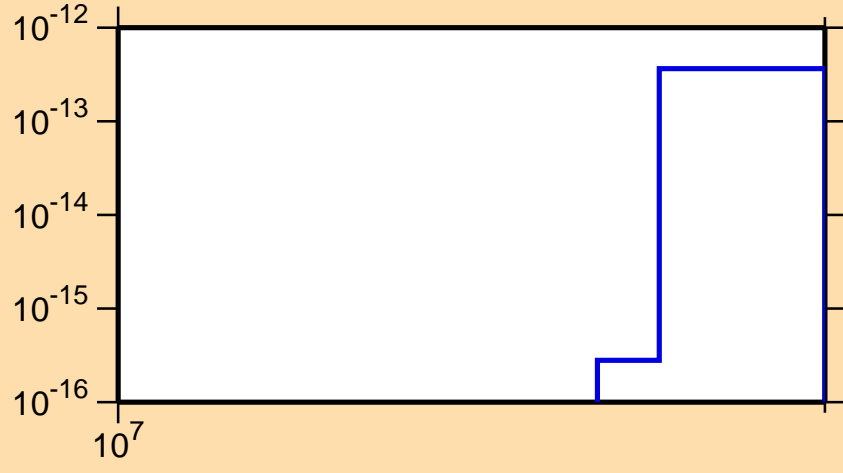
\sigma vs. E for ^{140}\text{Ba} (mt 45)
