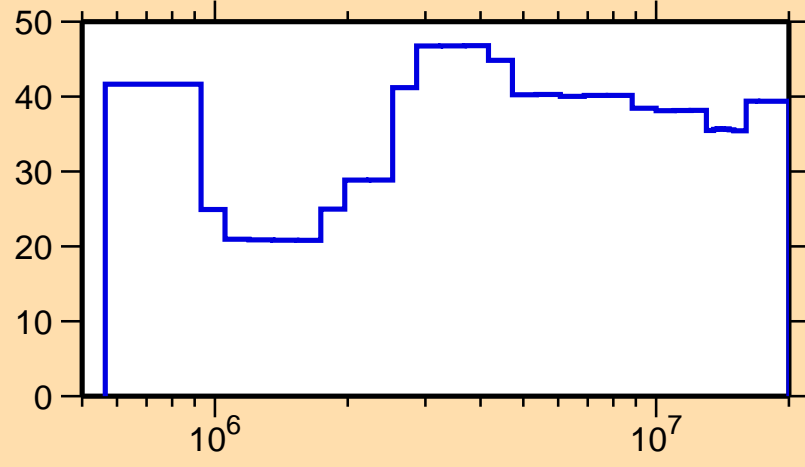
\Delta\sigma/\sigma vs. E for ^{140}\text{Ba}(n,n_1)
