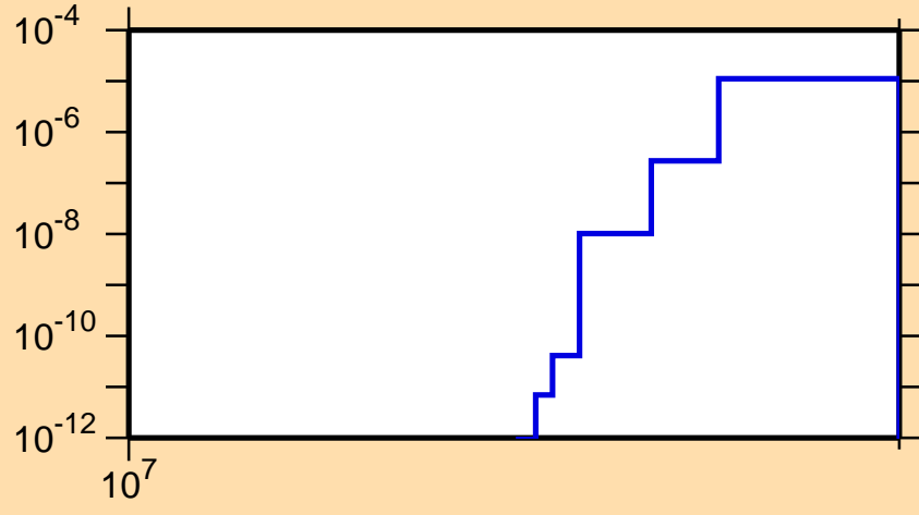
\sigma vs. E for ^{140}\text{Ba}(n,nt)
