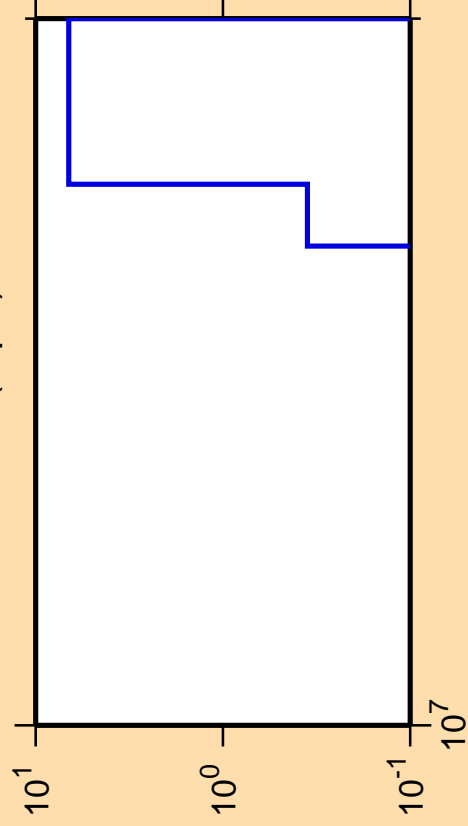
\Delta\sigma/\sigma vs. E for ^{140}\text{Ba}(n,p\alpha)
