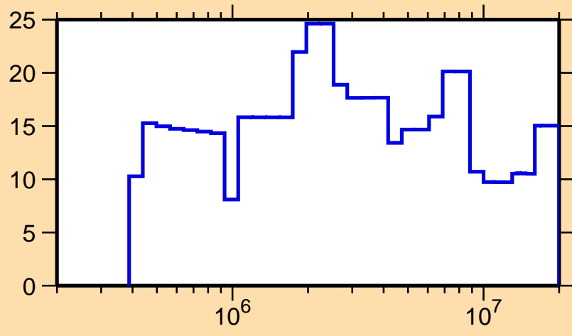
\Delta\sigma/\sigma vs. E for ^{140}\text{Ba}(n,\text{el.})
