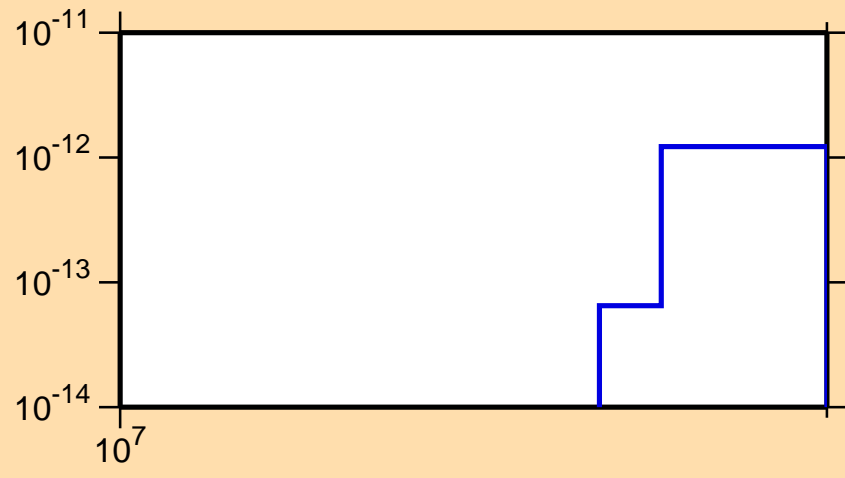
\sigma vs. E for ^{140}\text{Ba}(n,p\alpha)
