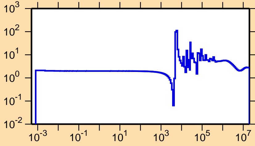
\sigma vs. E for ^{140}\text{Ba}(n,\text{el.})
