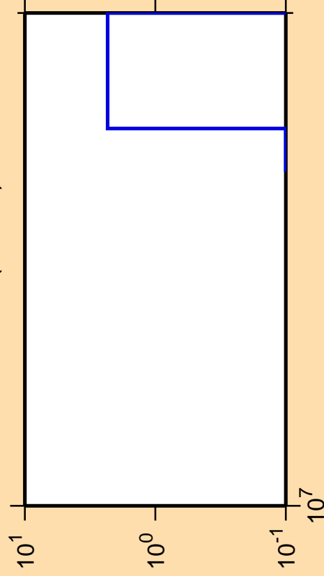
\Delta\sigma/\sigma vs. E for ^{140}\text{Ba}(n,\text{He}3)
