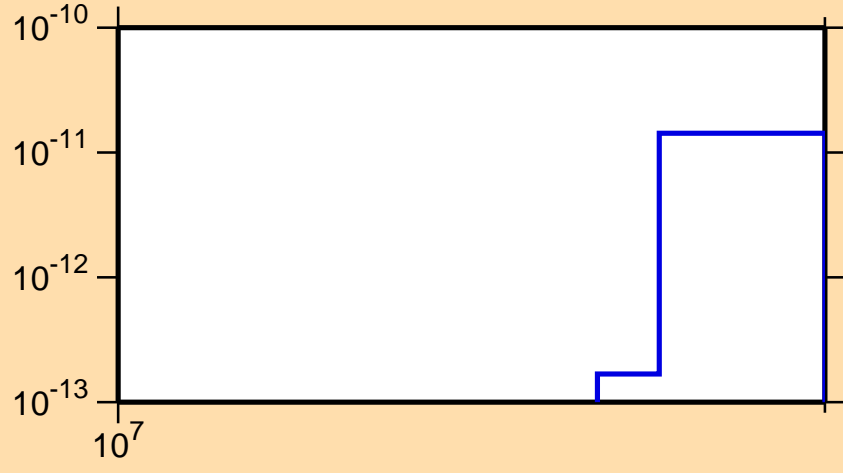
\sigma vs. E for ^{140}\text{Ba}(\text{mt117})
