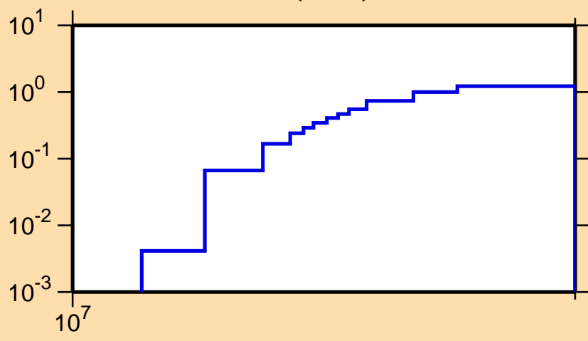
\sigma vs. E for ^{140}\text{Ba}(n,3n)
