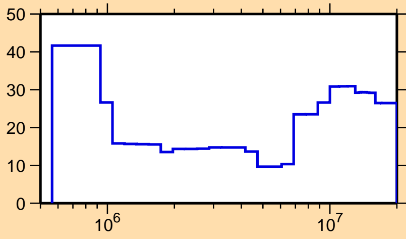
\Delta\sigma/\sigma vs. E for ^{140}\text{Ba}(n,\text{inel.})
