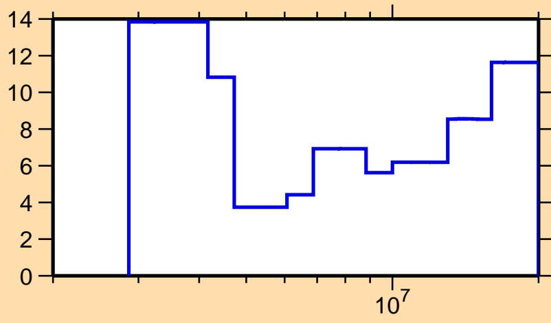
\Delta\sigma/\sigma vs. E for ^{140}\text{Ba}(n,\text{tot.})
