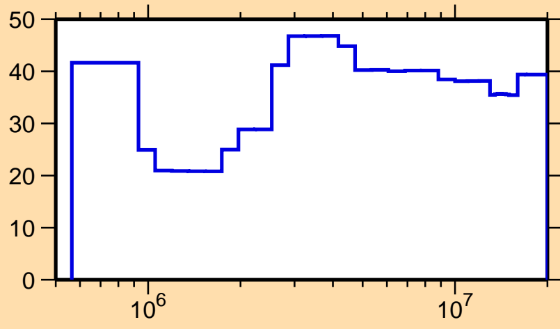
\Delta\sigma/\sigma vs. E for ^{140}\text{Ba}(n,n_1)
