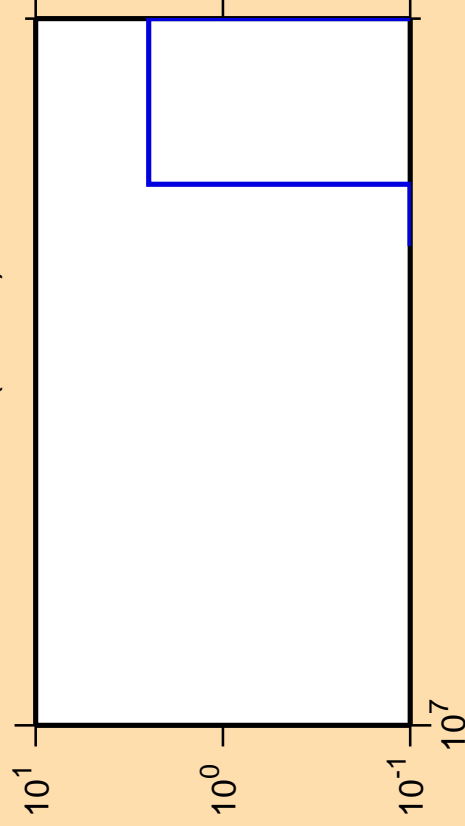
\Delta\sigma/\sigma vs. E for ^{140}\text{Ba} (mt 45)
