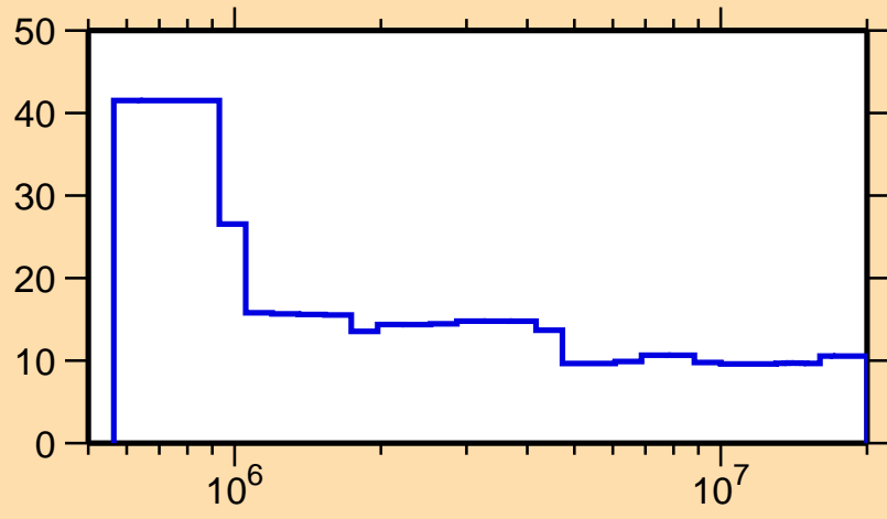
\Delta\sigma/\sigma vs. E for ^{140}\text{Ba}(n,\text{nonel.})
