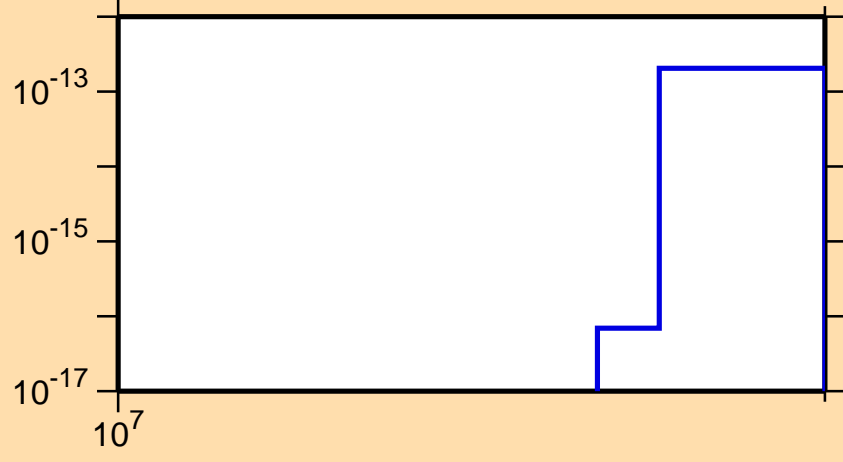
\sigma vs. E for ^{140}\text{Ba}(n,3n\alpha)
