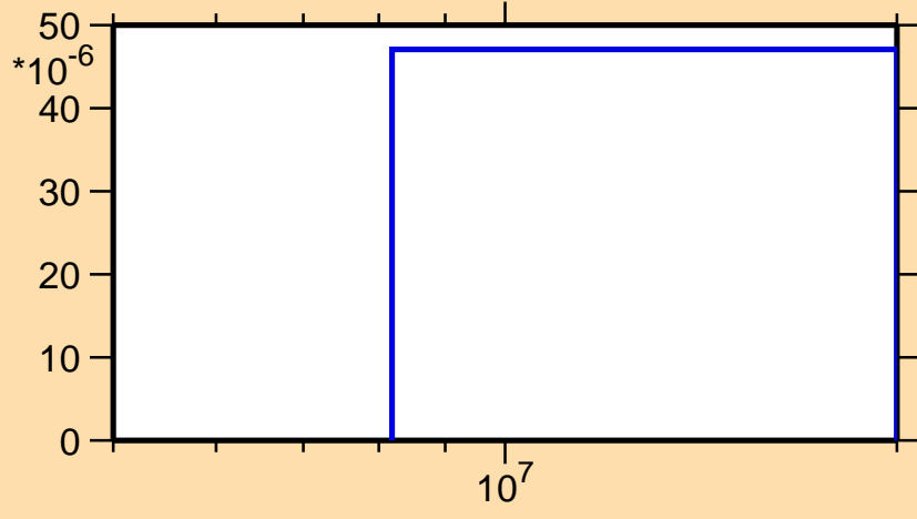
\sigma vs. E for ^{140}\text{Ba}(n,d)
