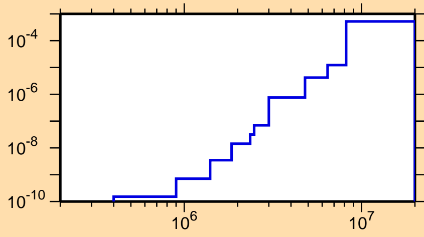
\sigma vs. E for ^{140}\text{Ba}(n,\alpha)
