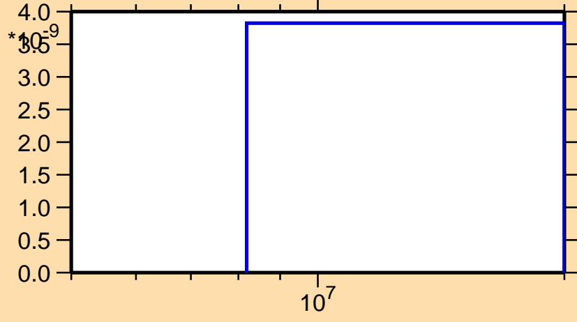
\sigma vs. E for ^{140}\text{Ba}(n,\text{nd})
