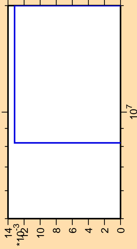
\Delta\sigma/\sigma vs. E for ^{140}\text{Ba}(n,3n\alpha)
