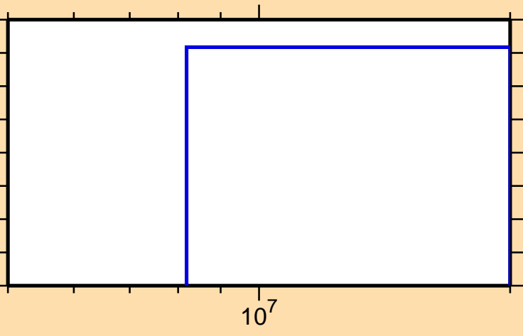
\sigma vs. E for ^{140}\text{Ba}(n,t)
