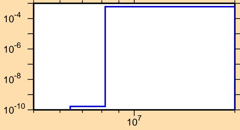
\sigma vs. E for ^{140}\text{Ba}(n,p)
