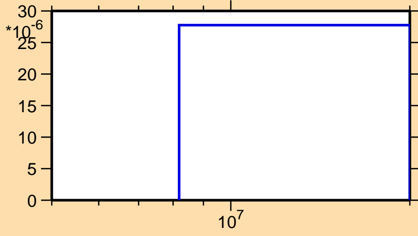
\sigma vs. E for ^{140}\text{Ba}(n,np)
