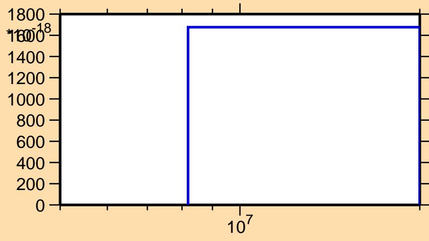
\sigma vs. E for ^{140}\text{Ba}(n,3n\alpha)
