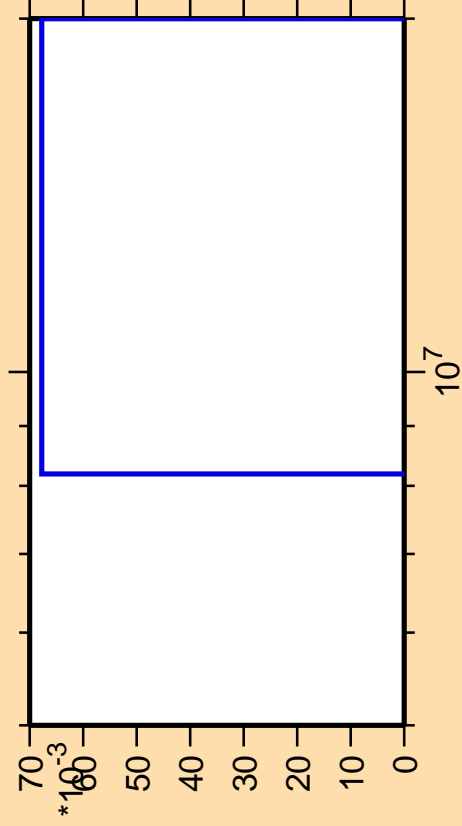
\Delta\sigma/\sigma vs. E for ^{140}\text{Ba}(n,p\alpha)
