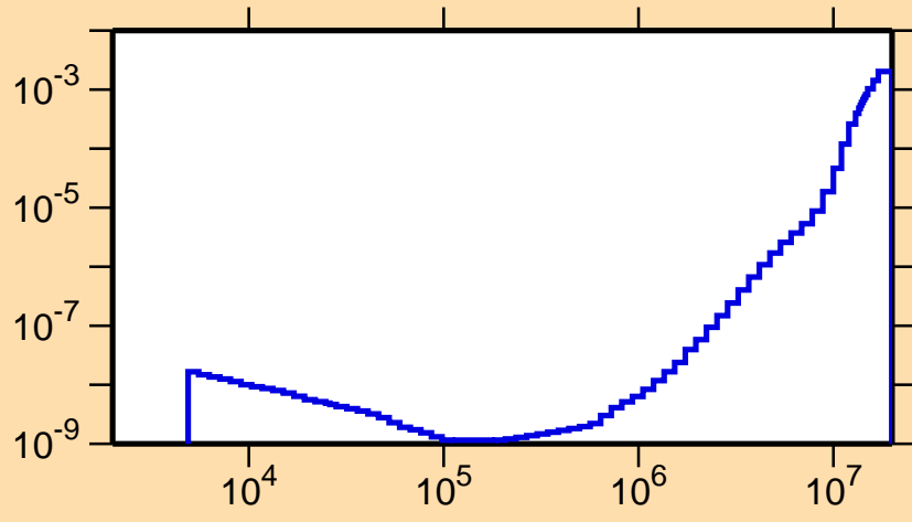
\sigma vs. E for ^{141}\text{Ba}(n,\alpha)
