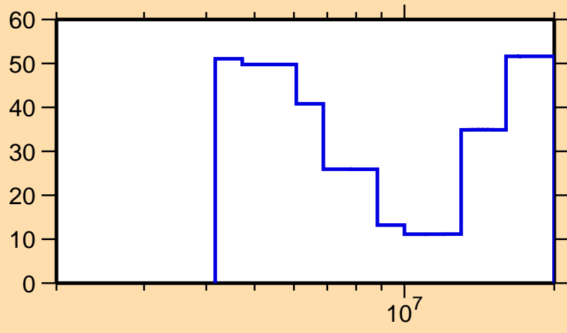
\Delta\sigma/\sigma vs. E for ^{141}\text{Ba}(n,2n)
