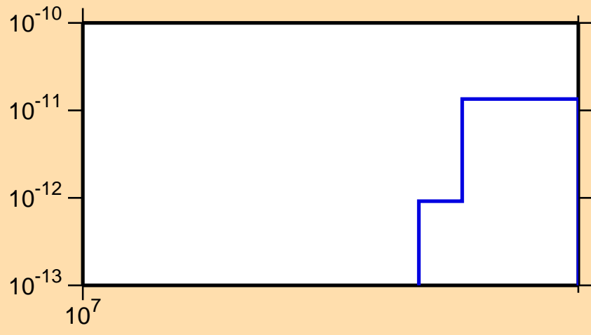
\sigma vs. E for ^{141}\text{Ba}(n,p\alpha)
