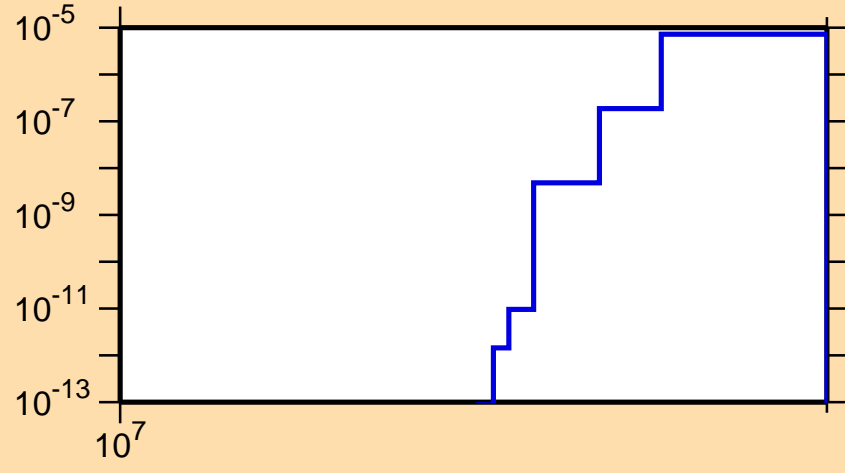
\sigma vs. E for ^{141}\text{Ba}(n,\text{nd})
