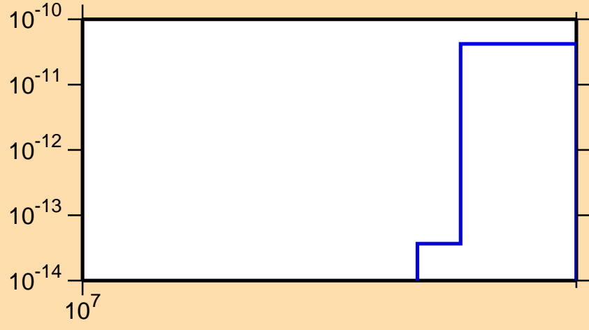
\sigma vs. E for ^{141}\text{Ba}(n,3n\alpha)
