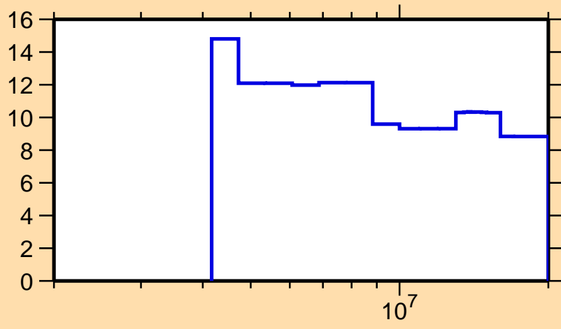
\Delta\sigma/\sigma vs. E for ^{141}\text{Ba}(n,\text{nonel.})
