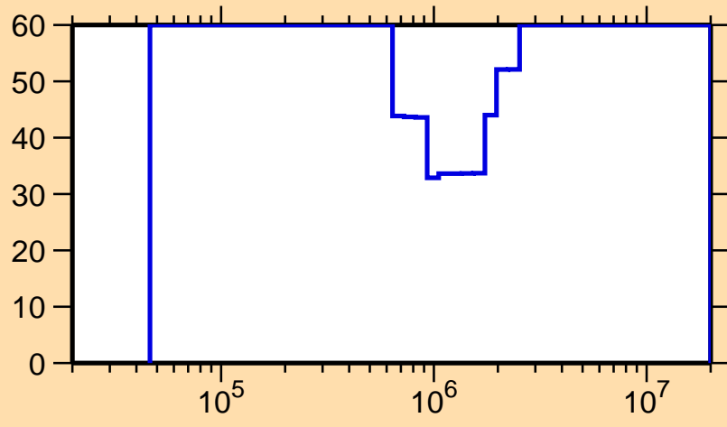
\Delta\sigma/\sigma vs. E for ^{141}\text{Ba}(n,n_1)
