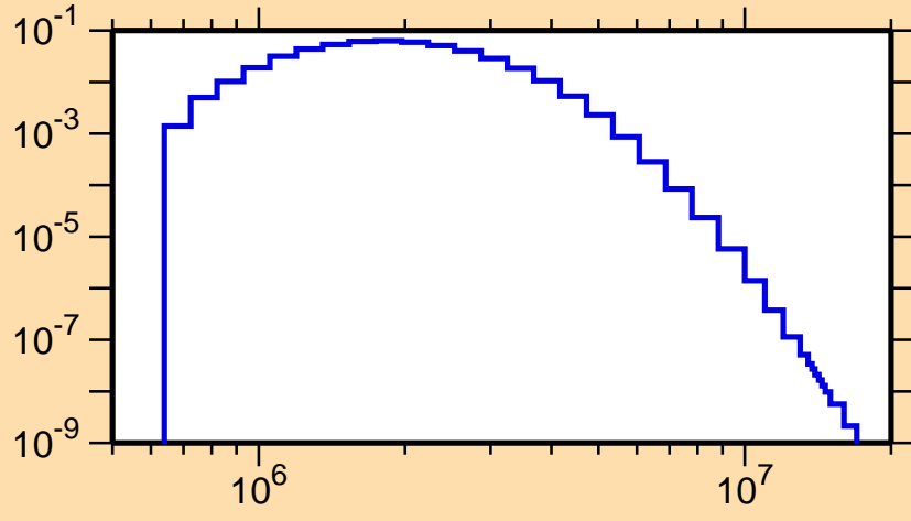
\sigma vs. E for ^{141}\text{Ba}(n,n_4)
