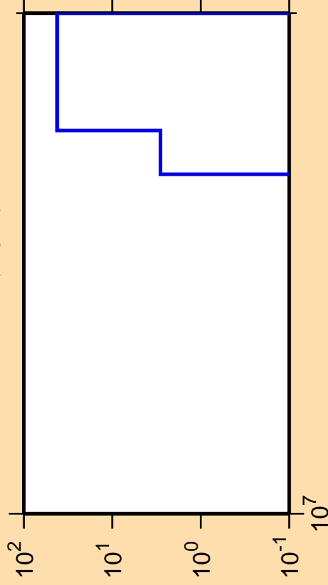
\Delta\sigma/\sigma vs. E for ^{141}\text{Ba}(n,p\alpha)
