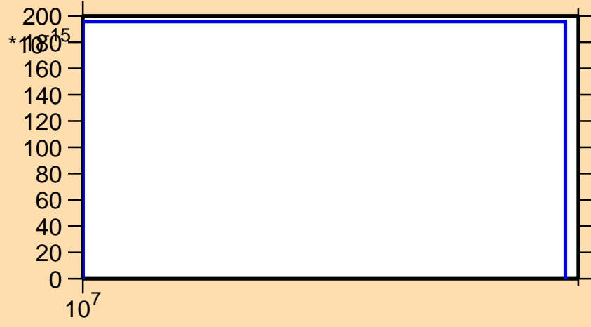
\sigma vs. E for ^{141}\text{Ba}(n,p\alpha)
