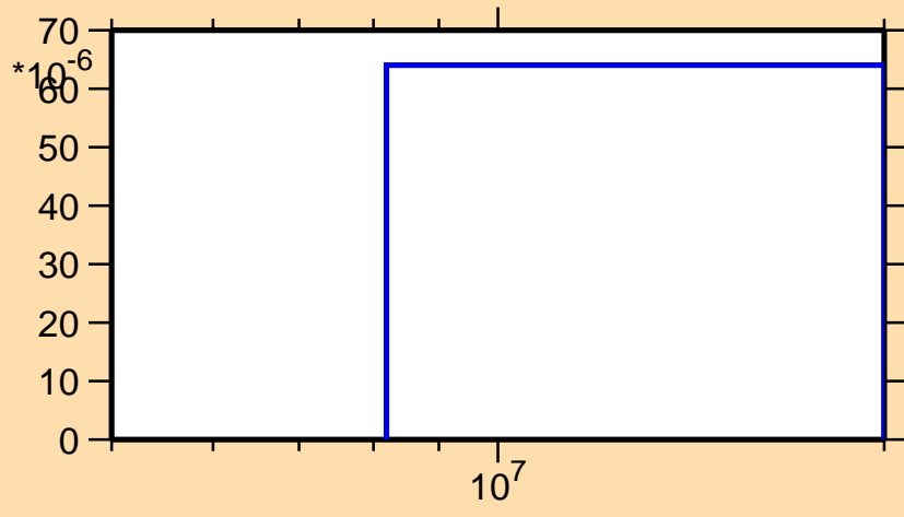
\sigma vs. E for ^{141}\text{Ba}(n,d)
