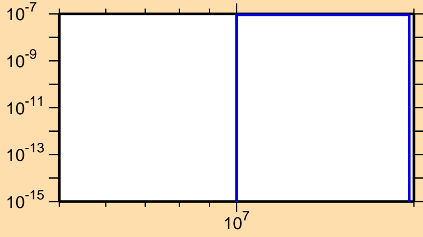
\sigma vs. E for ^{142}\text{Ba}(n,2n\alpha)
