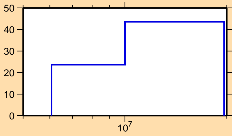
\Delta\sigma/\sigma vs. E for ^{142}\text{Ba}(n,n\text{cont.})
