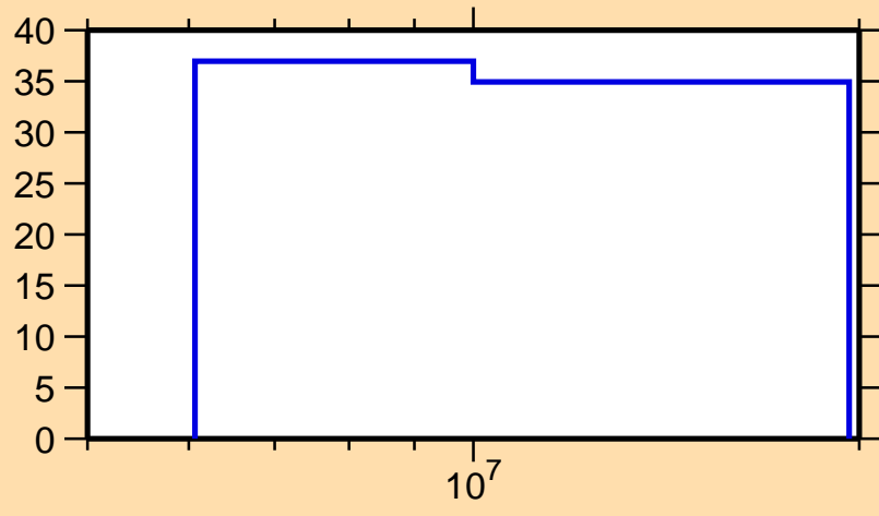
\Delta\sigma/\sigma vs. E for ^{142}\text{Ba}(n,n_1)
