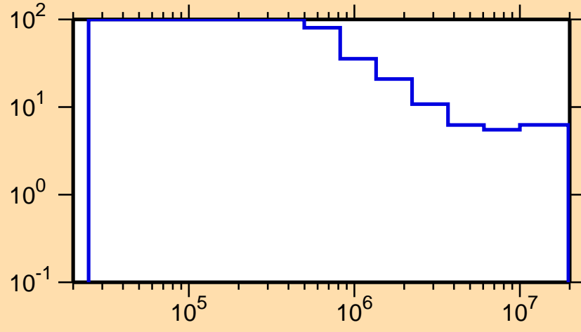
\Delta\sigma/\sigma vs. E for ^{142}\text{Ba}(n,\text{nonel.})
