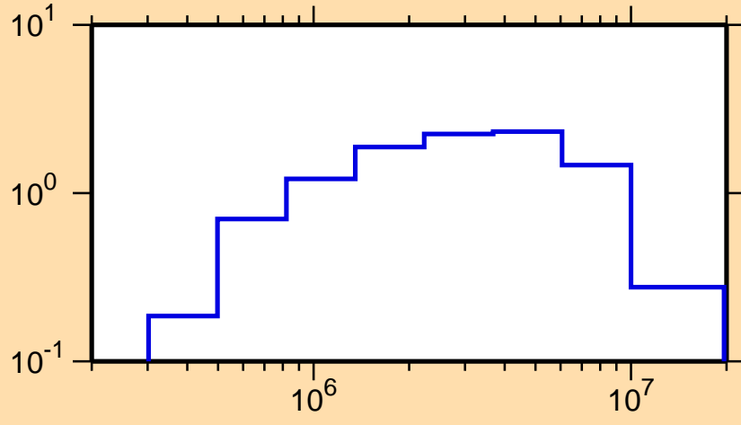
\sigma vs. E for ^{142}\text{Ba}(n,\text{inel.})
