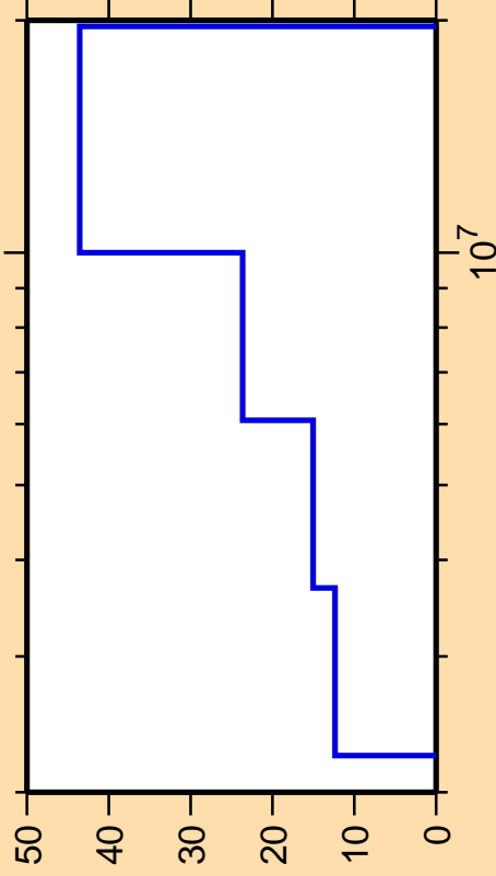
\Delta\sigma/\sigma vs. E for ^{142}\text{Ba}(n,n\text{cont.})
