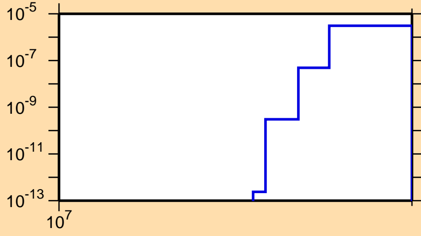
\sigma vs. E for ^{143}\text{Ba}(n,\text{nd})
