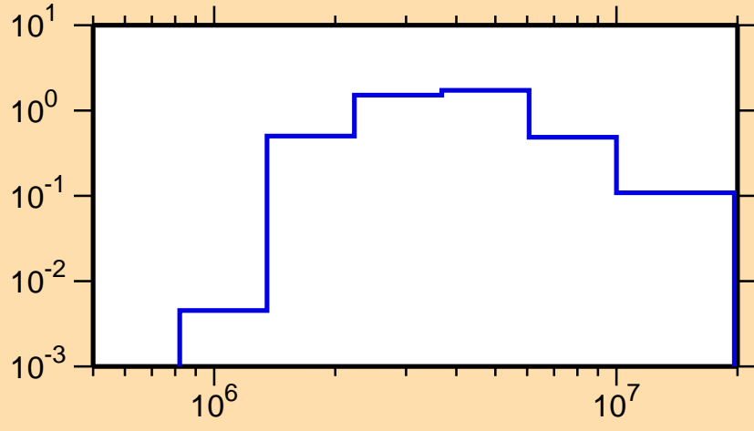
\sigma vs. E for ^{143}\text{Ba}(n,n\text{cont.})
