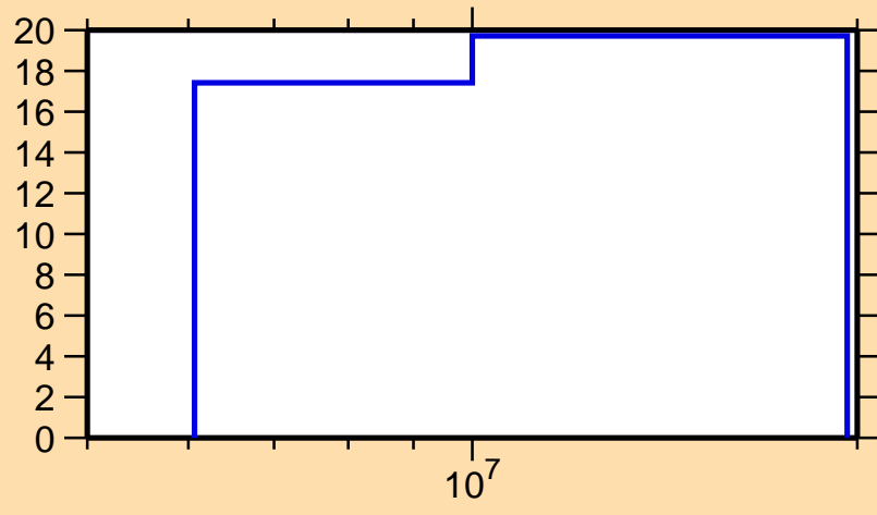
\Delta\sigma/\sigma vs. E for ^{143}\text{Ba}(n,\text{nonel.})
