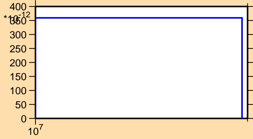
\sigma vs. E for ^{143}\text{Ba}(n,2np)
