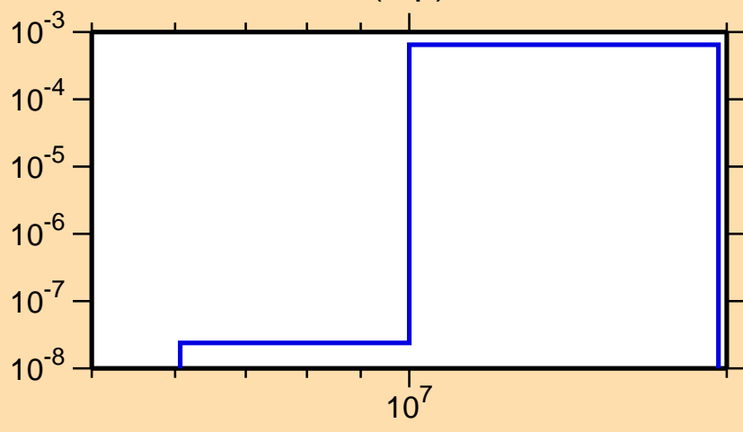
\sigma vs. E for ^{143}\text{Ba}(n,p)
