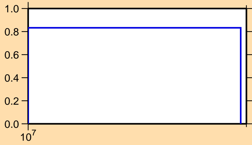
\sigma vs. E for ^{143}\text{Ba}(n,3n)
