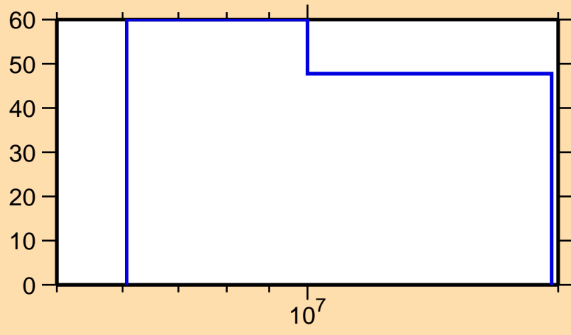
\Delta\sigma/\sigma vs. E for ^{143}\text{Ba}(n,el.)
