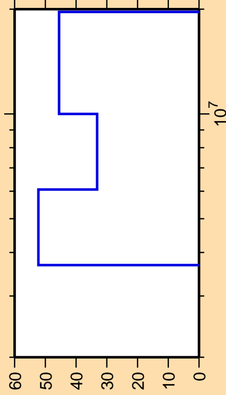
\Delta\sigma/\sigma vs. E for ^{143}\text{Ba}(n,2n)
