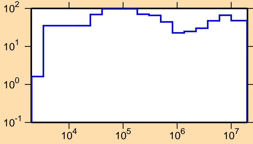
\Delta\sigma/\sigma vs. E for ^{143}\text{Ba}(n,\text{el.})
