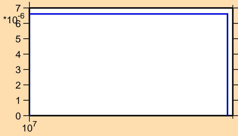
\sigma vs. E for ^{143}\text{Ba}(n,np)
