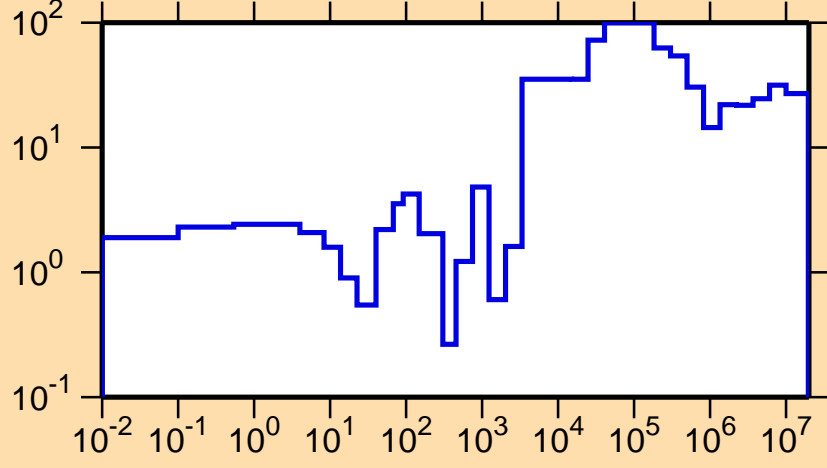
\Delta\sigma/\sigma vs. E for ^{143}\text{Ba}(n,\text{tot.})
