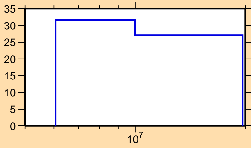
\Delta\sigma/\sigma vs. E for ^{143}\text{Ba}(n,\text{tot.})
