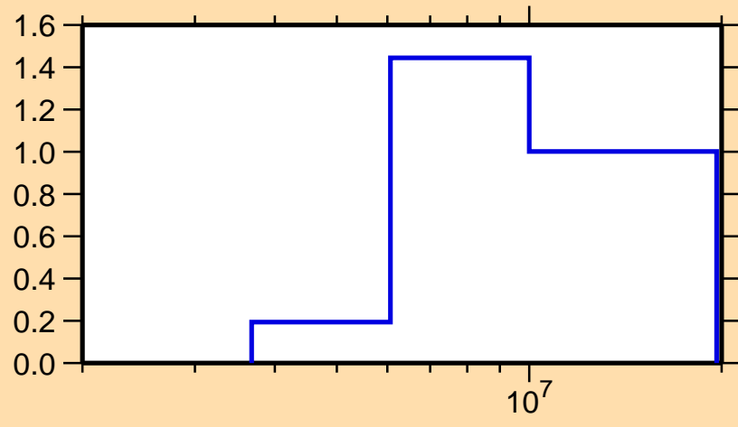
\sigma vs. E for ^{143}\text{Ba}(n,2n)
