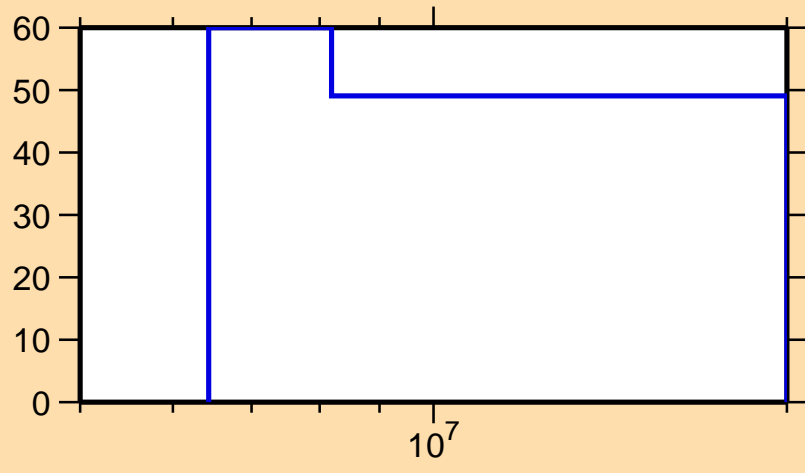
\Delta\sigma/\sigma vs. E for ^{143}\text{Ba}(n,\text{el.})
