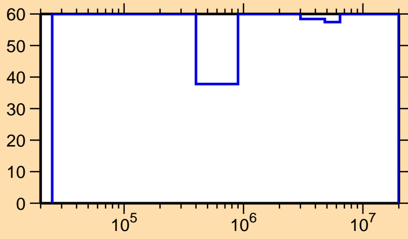
\Delta\sigma/\sigma vs. E for ^{143}\text{Ba}(n,n_1)
