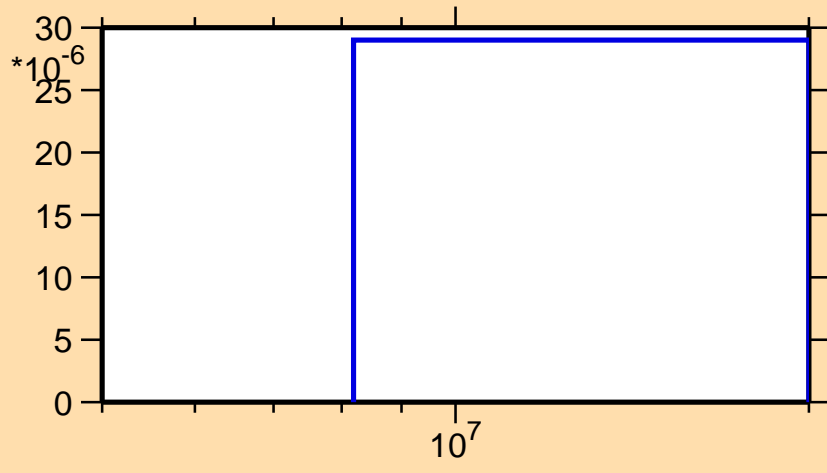
\sigma vs. E for ^{143}\text{Ba}(n,t)
