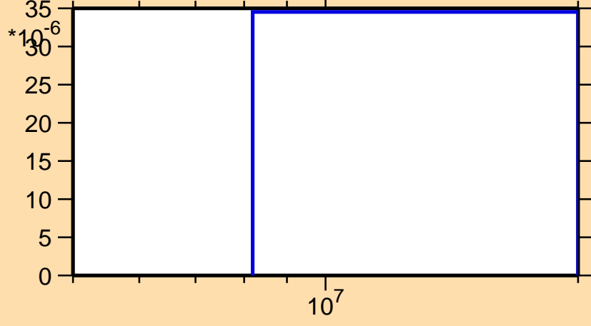
\sigma vs. E for ^{143}\text{Ba}(n,d)
