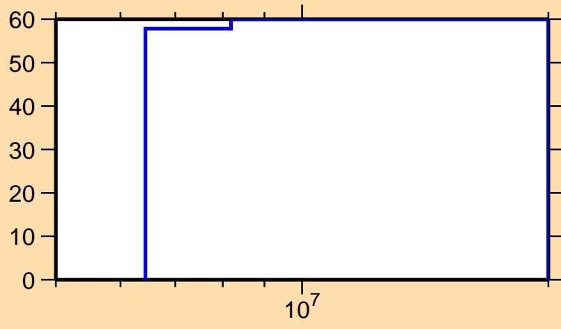
\Delta\sigma/\sigma vs. E for ^{143}\text{Ba}(n,p)
