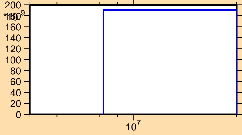
\sigma vs. E for ^{143}\text{Ba}(n,2n\alpha)
