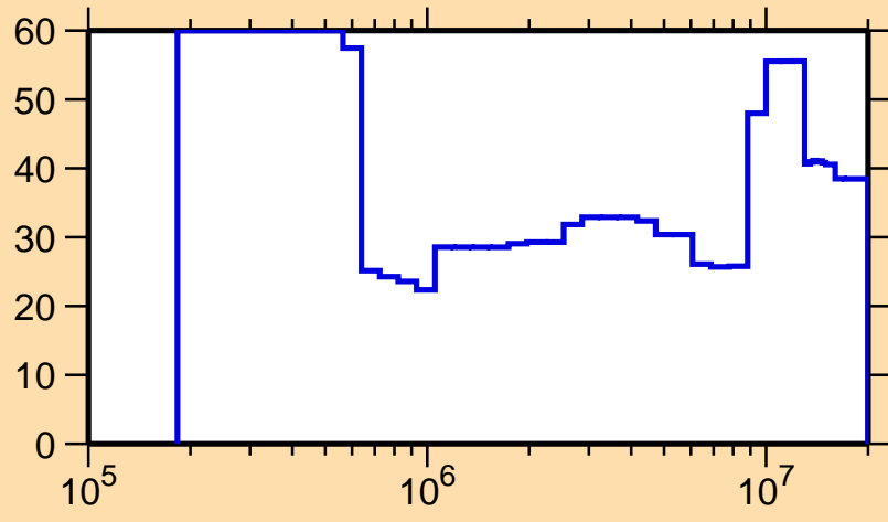
\Delta\sigma/\sigma vs. E for ^{144}\text{Ba}(n,\text{inel.})
