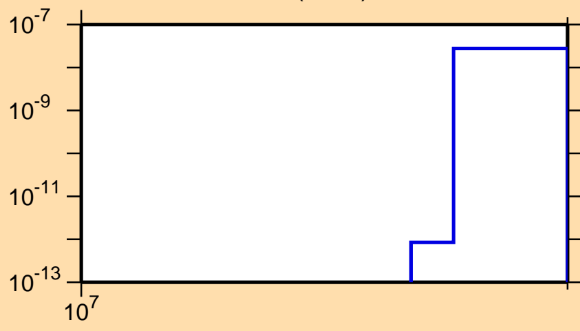
\sigma vs. E for ^{144}\text{Ba}(n,\text{nd})
