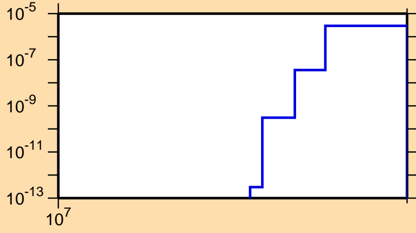
\sigma vs. E for ^{144}\text{Ba}(n,nt)
