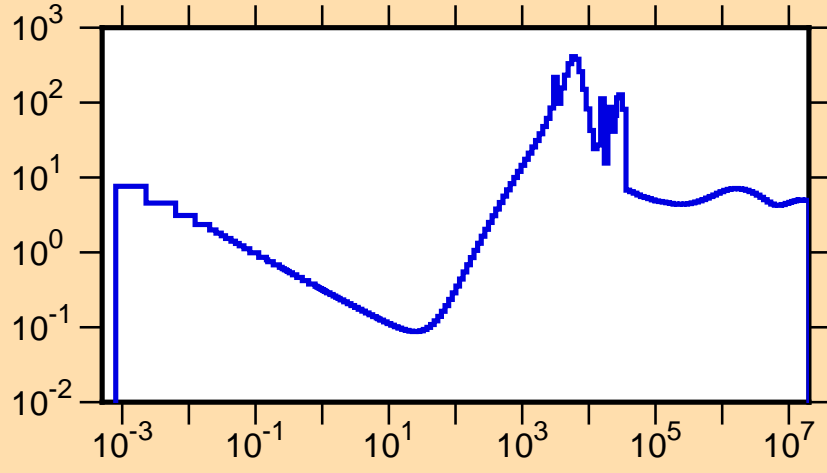
\sigma vs. E for ^{144}\text{Ba}(n,\text{tot.})
