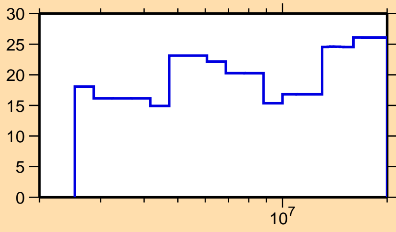
\Delta\sigma/\sigma vs. E for ^{144}\text{Ba}(n,\text{tot.})
