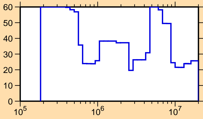
\Delta\sigma/\sigma vs. E for ^{144}\text{Ba}(n,\text{el.})
