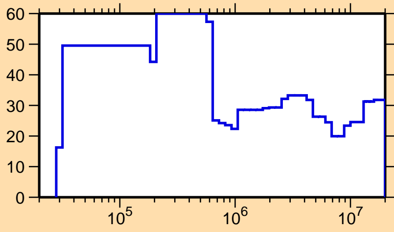
\Delta\sigma/\sigma vs. E for ^{144}\text{Ba}(n,\text{nonel.})
