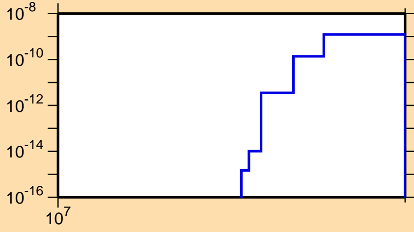
\sigma vs. E for ^{144}\text{Ba}(n,3n\alpha)
