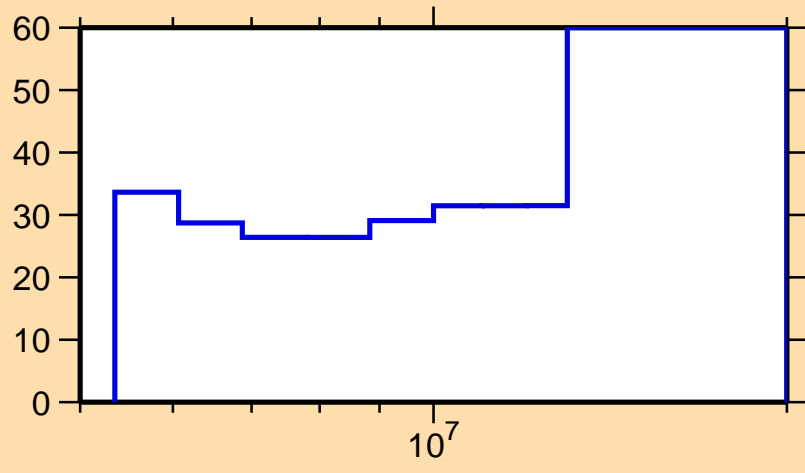
\Delta\sigma/\sigma vs. E for ^{144}\text{Ba}(n,2n)
