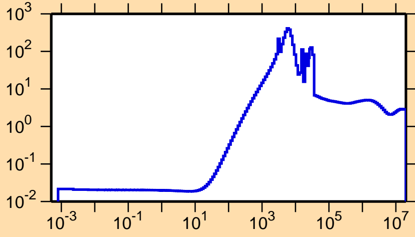
\sigma vs. E for ^{144}\text{Ba}(n,\text{el.})
