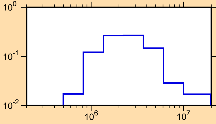
\sigma vs. E for ^{144}\text{Ba}(n,n_2)
