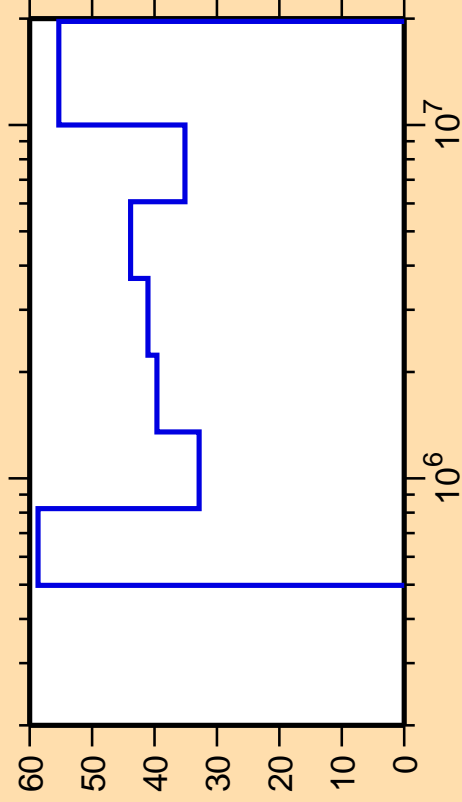
\Delta\sigma/\sigma vs. E for ^{144}\text{Ba}(n,n_2)
