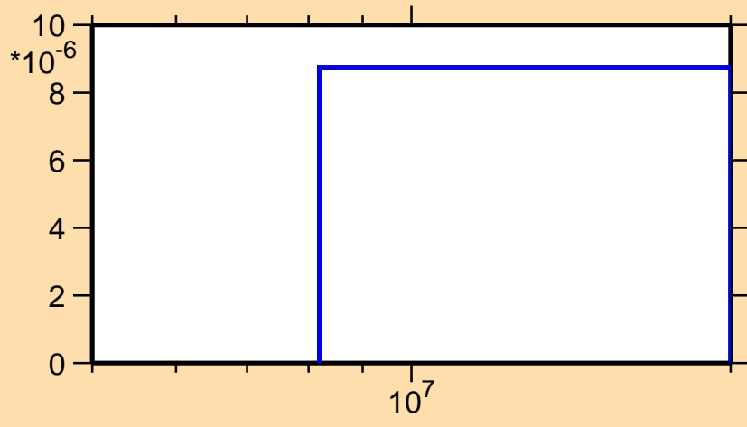
\sigma vs. E for ^{144}\text{Ba}(n,t)
