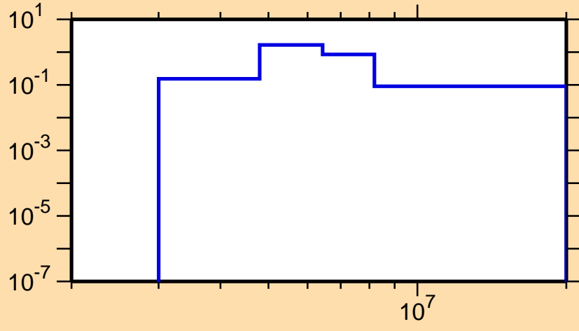
\sigma vs. E for ^{144}\text{Ba}(n,n\text{cont.})
