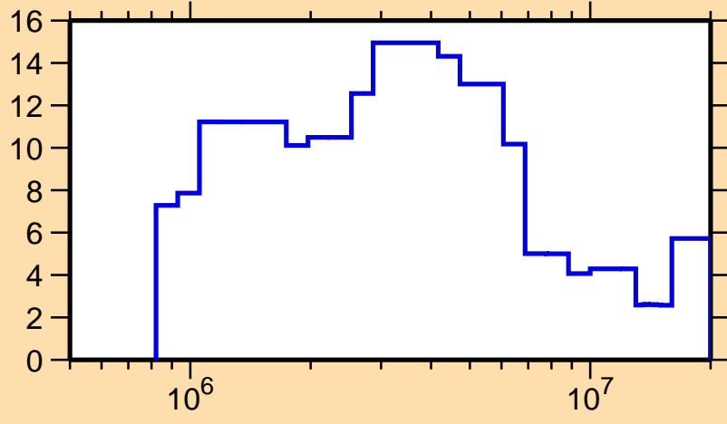
\Delta\sigma/\sigma vs. E for ^{145}\text{Ba}(n, tot.)
