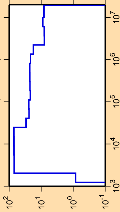
\Delta\sigma/\sigma vs. E for ^{145}\text{Ba}(n,\text{nonel.})
