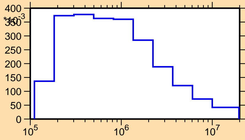
\sigma vs. E for ^{145}\text{Ba}(n,n_1)
