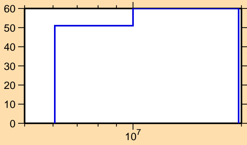
\Delta\sigma/\sigma vs. E for ^{145}\text{Ba}(n,\gamma)
