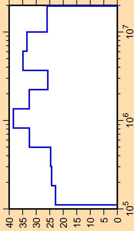
\Delta\sigma/\sigma vs. E for ^{145}\text{Ba}(n,n_1)
