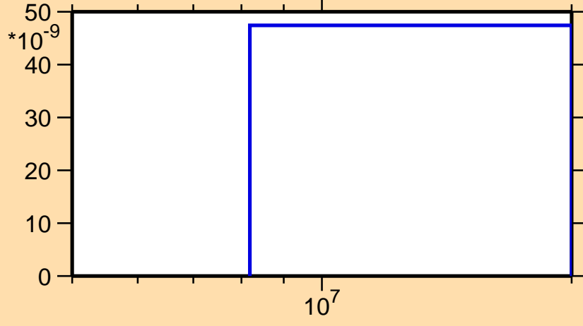
\sigma vs. E for ^{145}\text{Ba}(n,2n\alpha)
