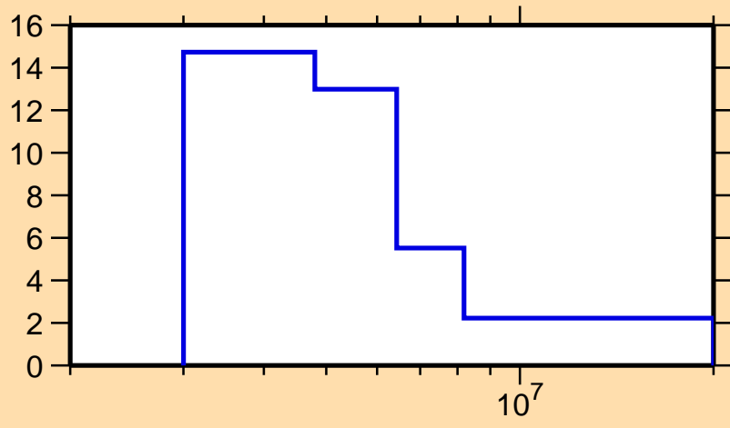
\Delta\sigma/\sigma vs. E for ^{145}\text{Ba}(n,\text{tot.})
