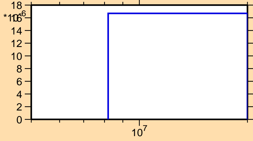
\sigma vs. E for ^{145}\text{Ba}(n,t)
