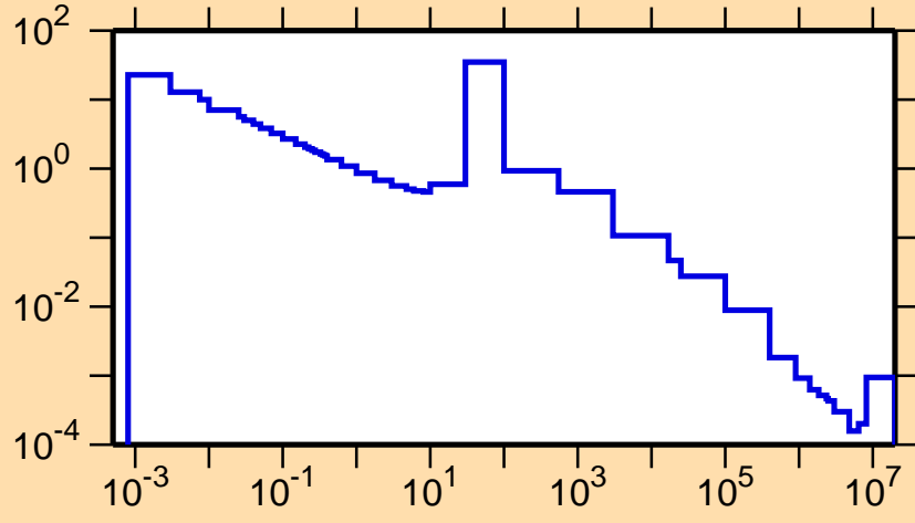
\sigma vs. E for ^{145}\text{Ba}(n,\gamma)
