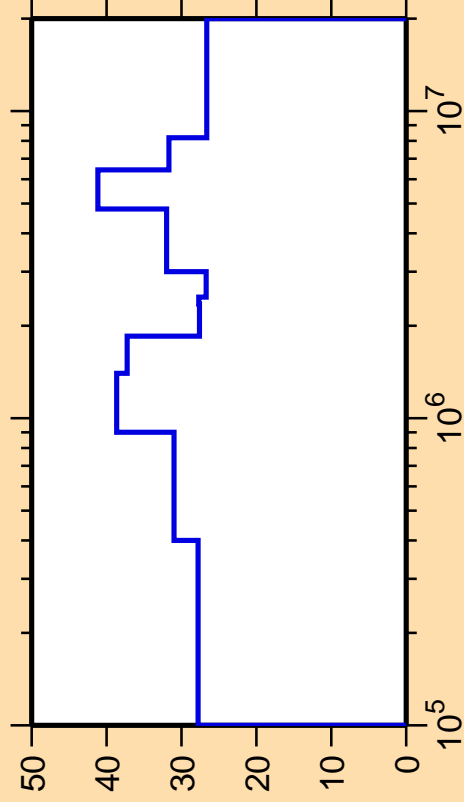
\Delta\sigma/\sigma vs. E for ^{145}\text{Ba}(n,n_2)
