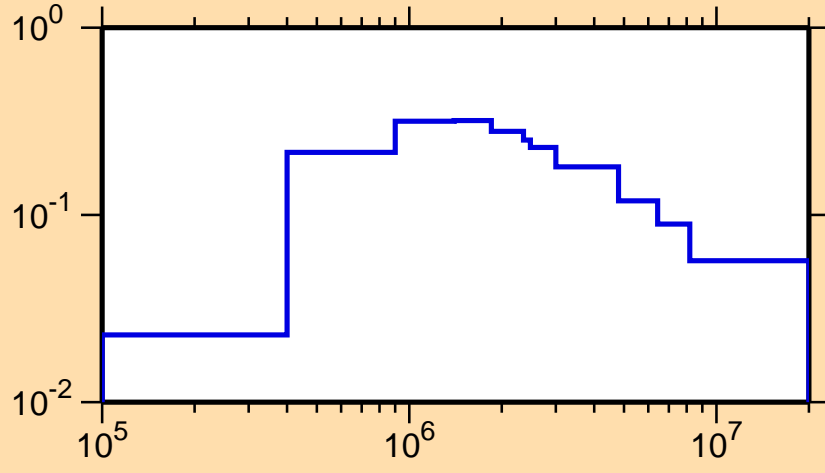
\sigma vs. E for ^{145}\text{Ba}(n,n_4)
