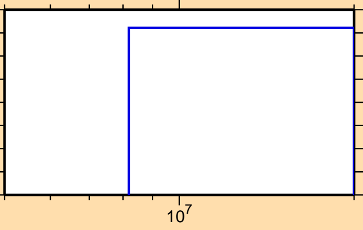
\sigma vs. E for ^{145}\text{Ba}(n,\text{nd})
