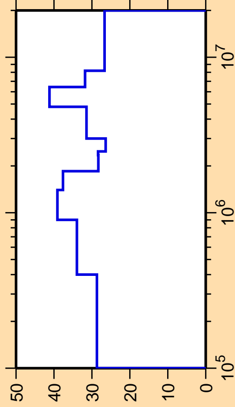
\Delta\sigma/\sigma vs. E for ^{145}\text{Ba}(n,n_4)
