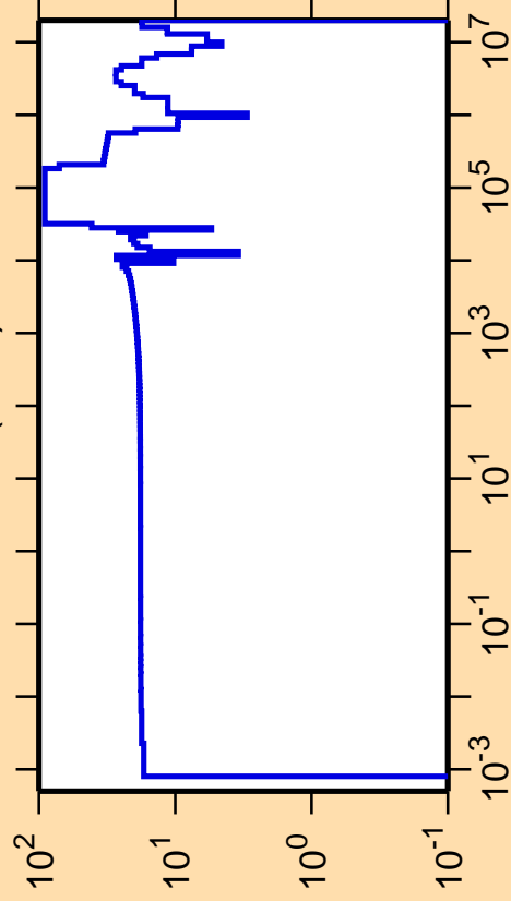
\Delta\sigma/\sigma vs. E for ^{146}\text{Ba}(n,\text{el.})
