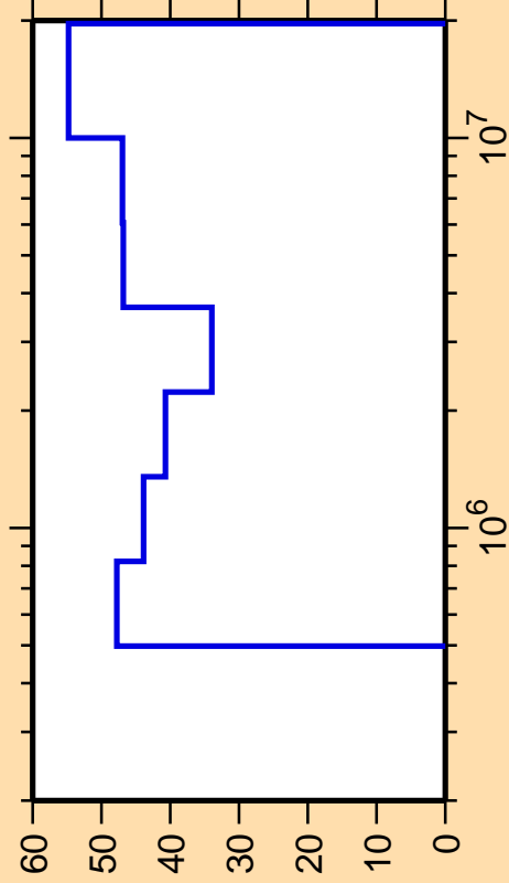
\Delta\sigma/\sigma vs. E for ^{146}\text{Ba}(n,n_3)
