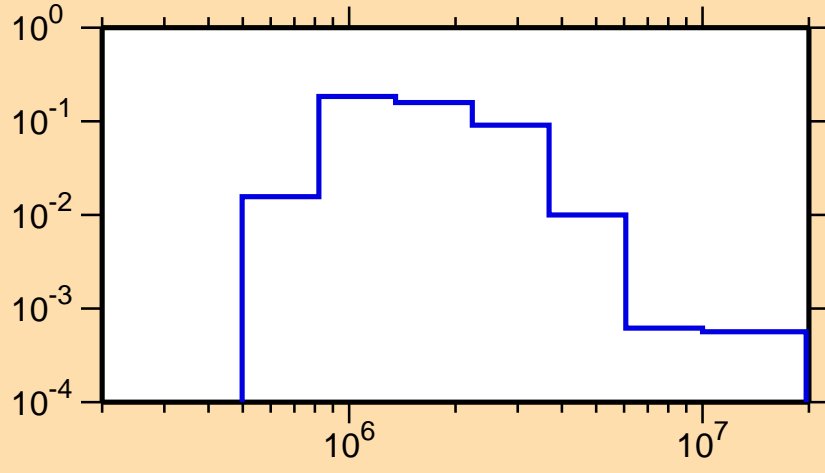
\sigma vs. E for ^{146}\text{Ba}(n,n_3)
