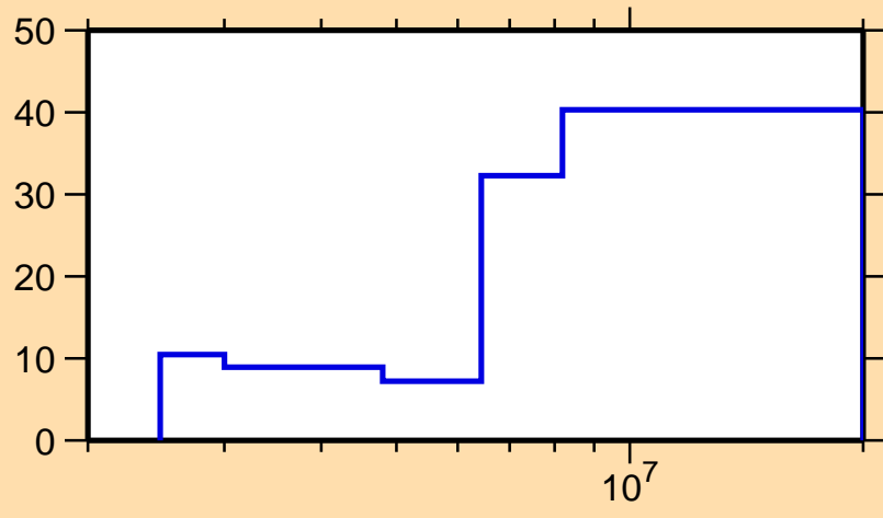
\Delta\sigma/\sigma vs. E for ^{146}\text{Ba}(n,\text{inel.})
