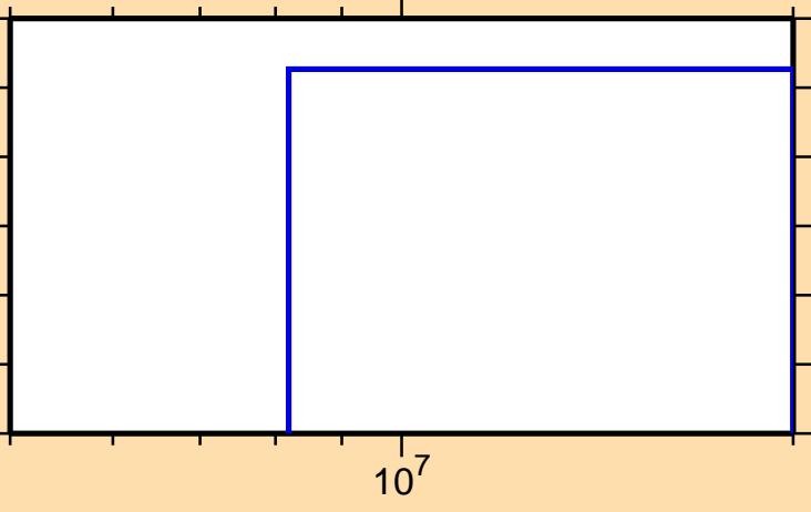
\sigma vs. E for ^{146}\text{Ba}(n,\text{nd})
