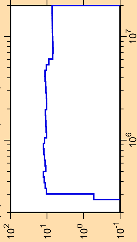
\Delta\mu/\mu vs. E for {}^7\text{Be}(\text{mt251})
