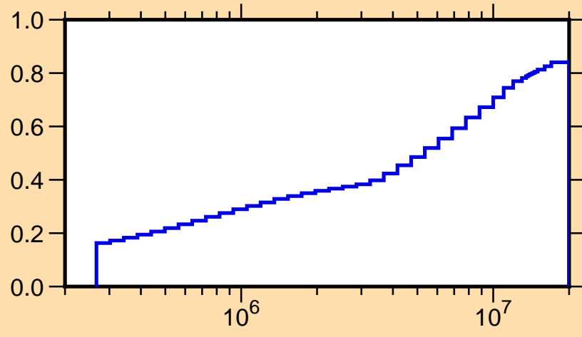
\mu vs. E for {}^7\text{Be}(\text{mt251})
