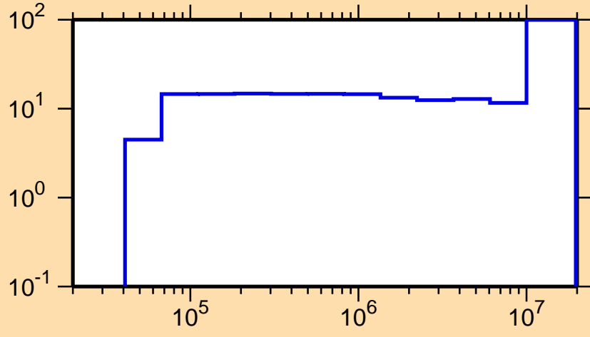
\Delta\sigma/\sigma vs. E for {}^7\text{Be}(n,p)
