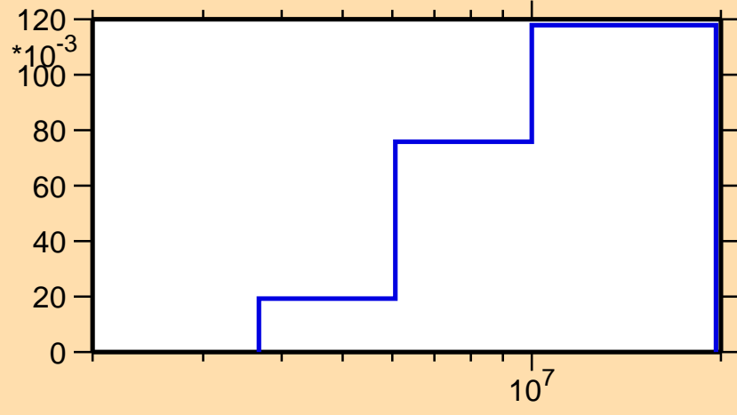
\sigma vs. E for {}^7\text{Be}(n,d)
