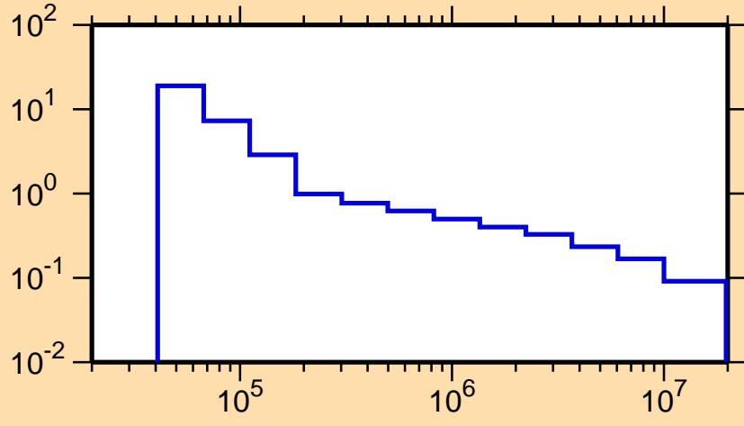
\sigma vs. E for {}^7\text{Be}(n,p)
