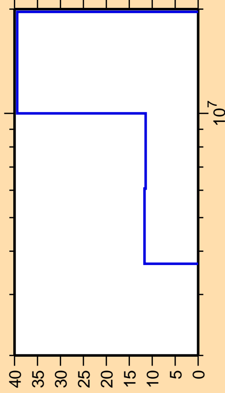
\Delta\sigma/\sigma vs. E for {}^7\text{Be}(n,d)
