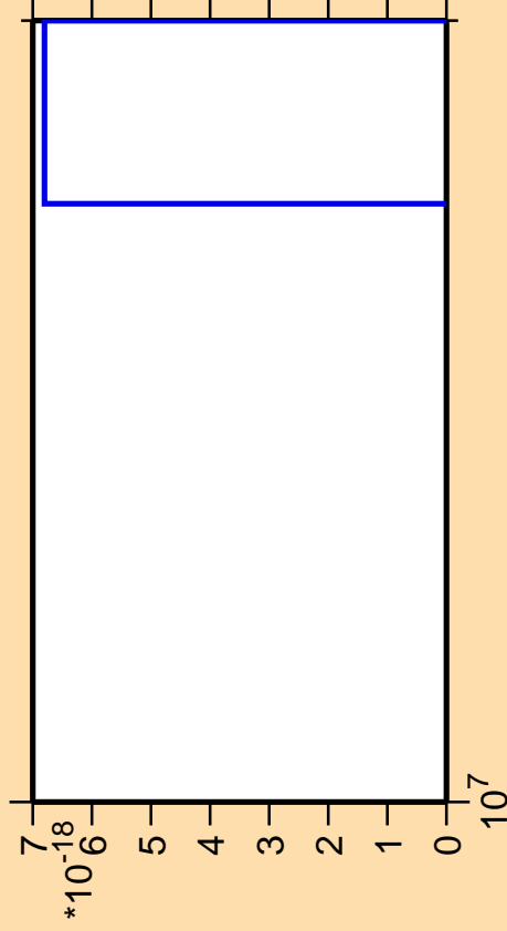
\Delta\sigma/\sigma vs. E for ^{11}\text{Be}(n,\alpha)
