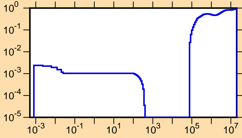
\mu vs. E for ^{271}
