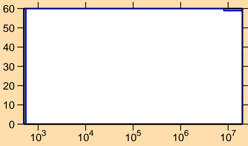
\Delta\sigma/\sigma vs. E for ^{271}\gamma
