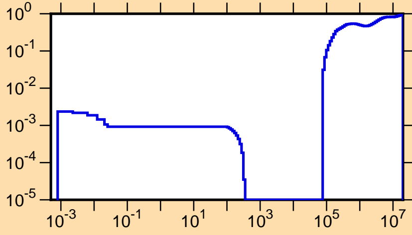
\mu vs. E for ^{274}
