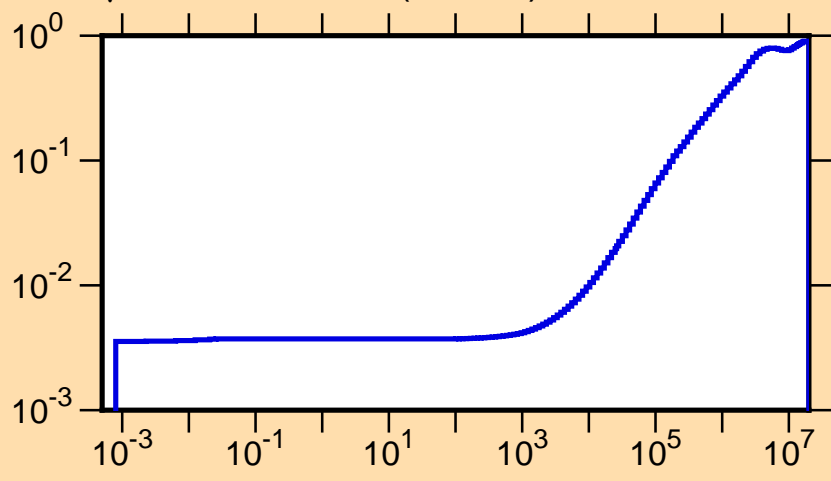
\mu vs. E for ^{190}\text{Bi}(\text{mt251})
