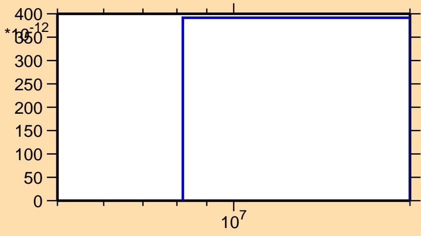
\sigma vs. E for ^{190}\text{Bi} (mt 34)
