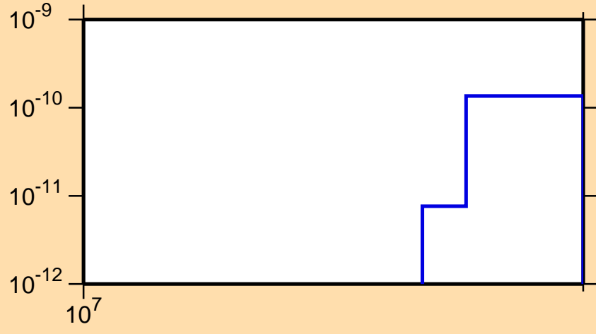
\sigma vs. E for ^{191}\text{Bi} (mt 34)
