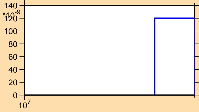
\sigma vs. E for ^{191}\text{Bi}(n,3n)
