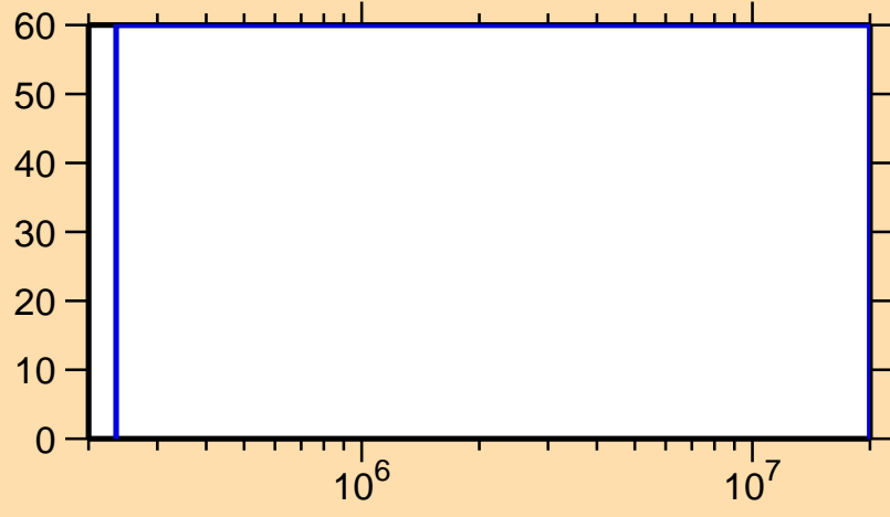
\Delta\sigma/\sigma vs. E for ^{191}\text{Bi}(n,n\text{cont.})
