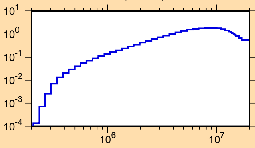
\sigma vs. E for ^{192}\text{Bi}(n,\text{inel.})
