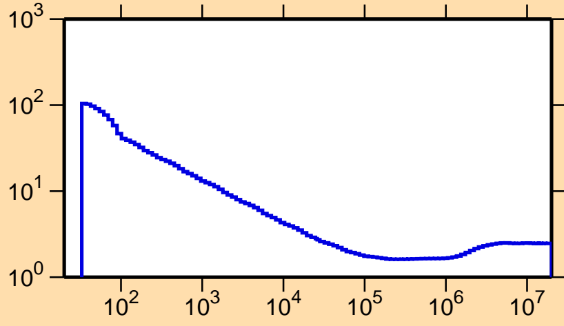
\sigma vs. E for ^{192}\text{Bi}(n,\text{nonel.})
